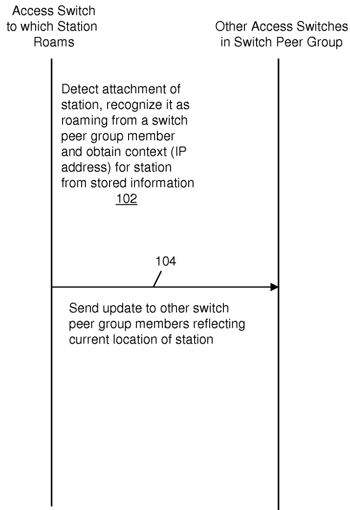
Control plane for roam within switch peer group
