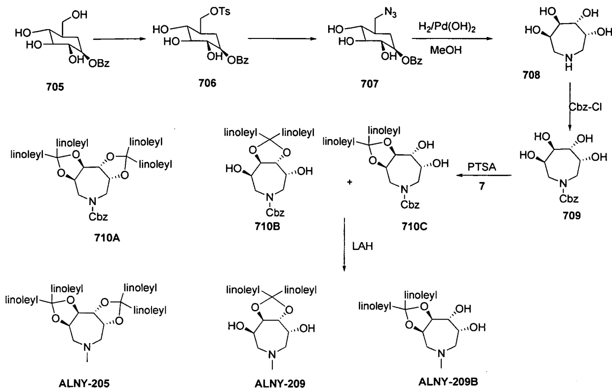
Scheme 22
