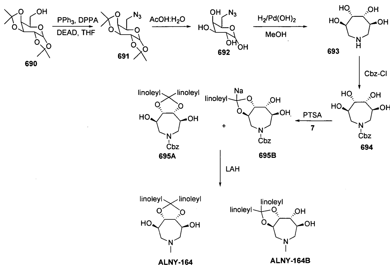
Scheme 20
