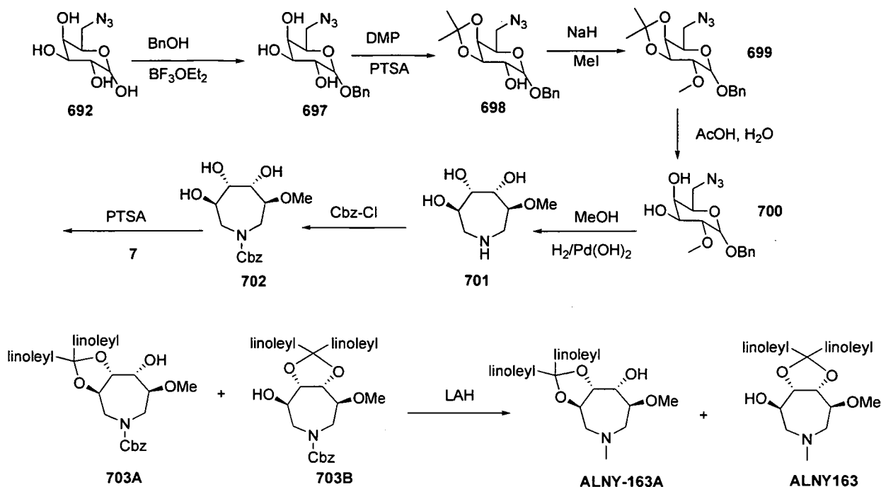
Scheme 21
