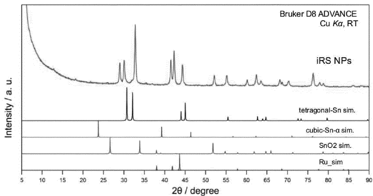
The PXRD pattern of iRS (Sn:Ru= 9:1)
