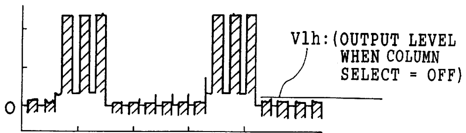
OUTPUT SIGNALS (RF AMPLIFIER INPUT SIGNALS)
