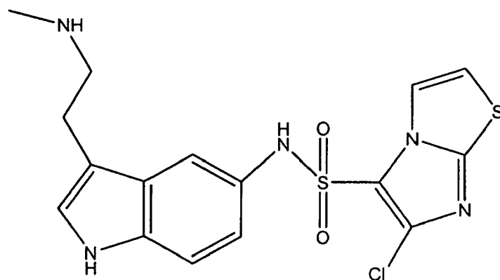
6-Chloro-imidazo[2,1- b ]thiazole-5-sulfonic acid [3-(2-methylamino-ethyl)-1 H -indol-5-yl]-amide
