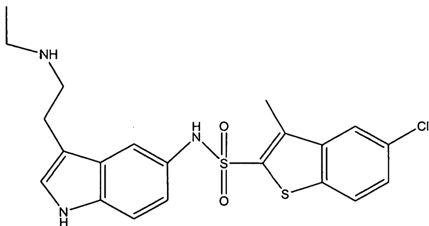
5-Chloro-3-methyl-benzo[b]thiophene-2-sulfonic acid [3-(2-ethylamino-ethyl)-1 H -indol-5-yl]-amide
