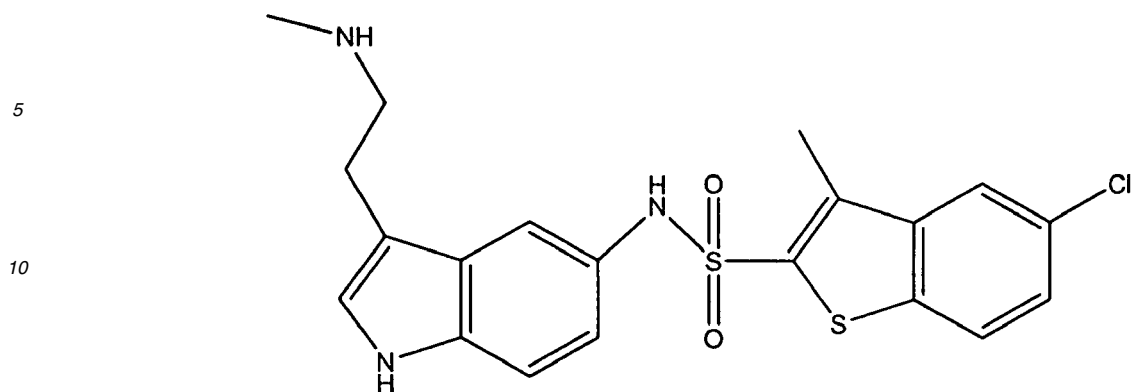
5-Chloro-3-methyl-benzo[b]thiophene-2-sulfonic acid [3-(2-methylamino-ethyl)-1H-indol-5-yl]-amide
