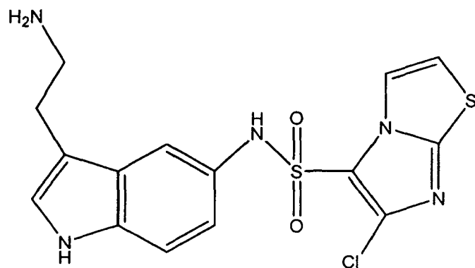
6-Chloro-imidazo[2,1- b ]thiazole-5-sulfonic acid [3-(2-amino-ethyl)-1 H -indol-5-yl]-amide
