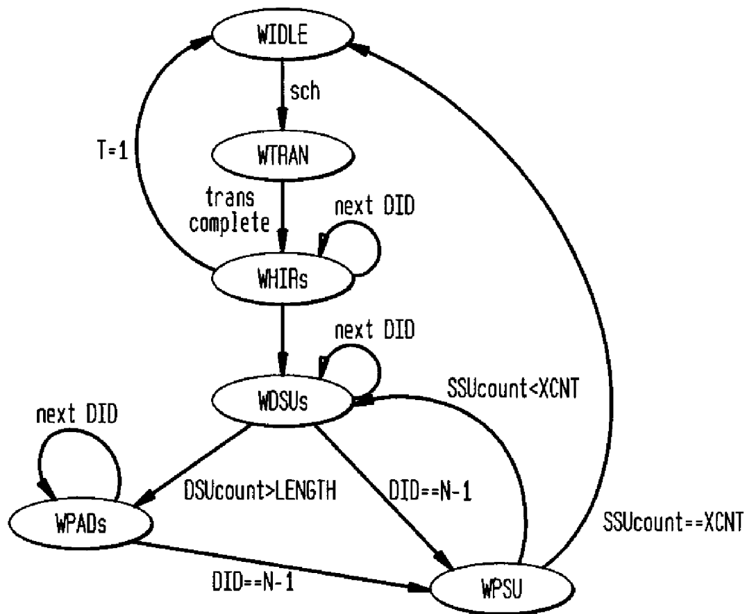
FIG. 24 WRITE OPERATION STATE MACHINE (WOSM) STATE DIAGRAM
