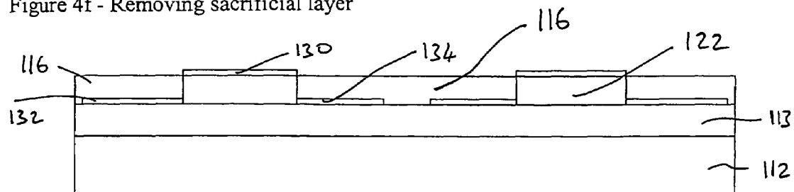
Figure 4f - Removing sacrificial layer
