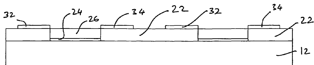
Figure 1f - Removing sacrificial layer
