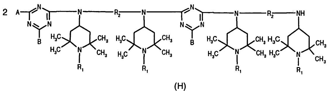
Scheme II-3:
