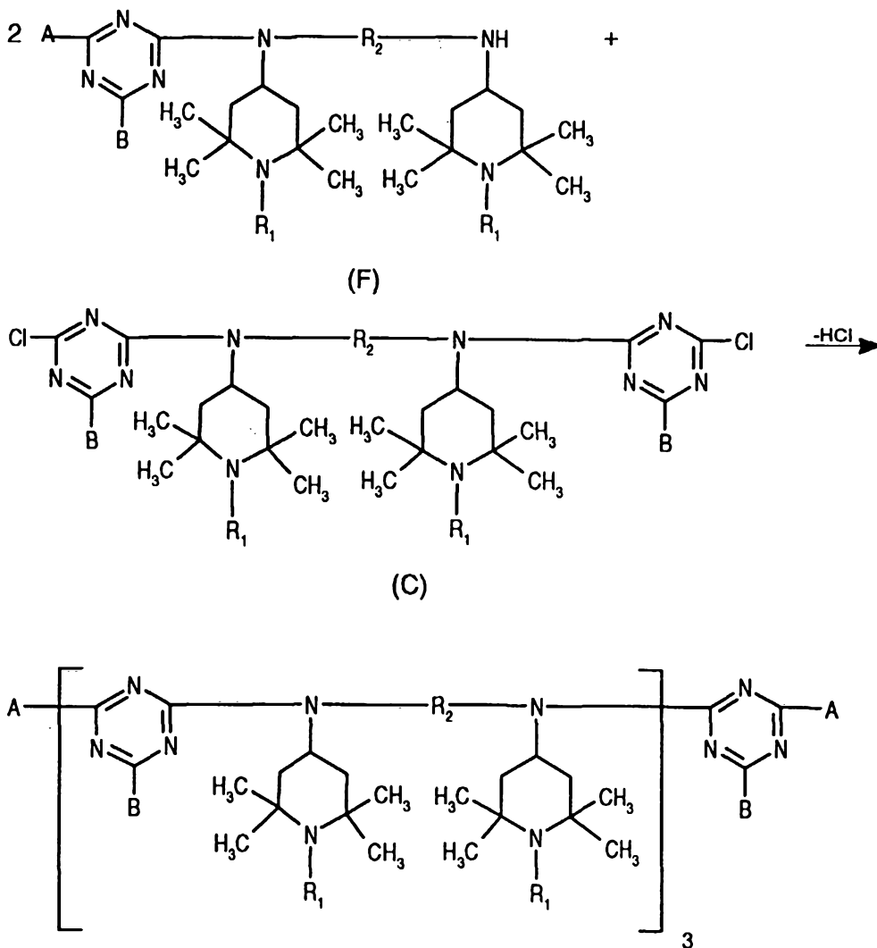
Scheme I-2:
