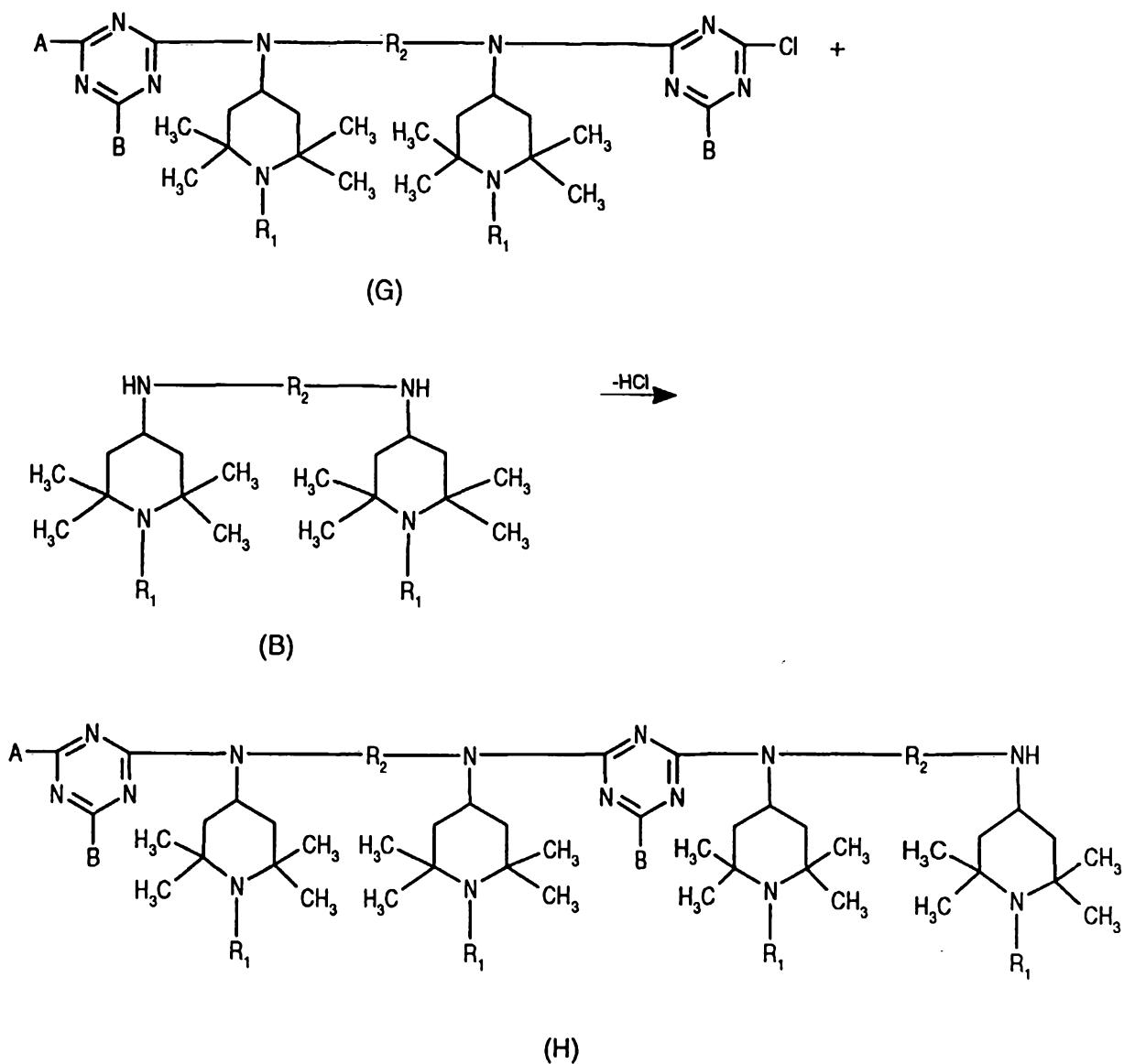
Scheme II-2:
