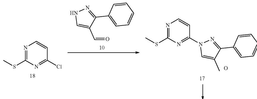
<Reaction Scheme 2>
