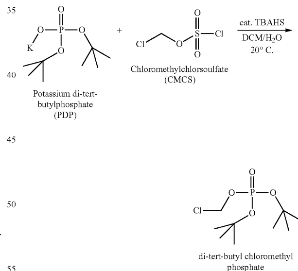
Scheme Ia
