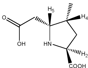
(2 S ,4 R ,5 S )-5-(carboxymethyl)-4-methylpyrrolidine-2-carboxylic acid
