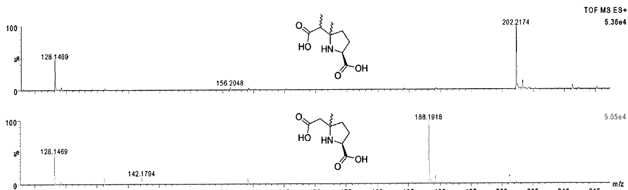
Figure 43: MS spectrum (positive ion electrospray ionization) for compound 24 (bottom) and compound 25 (top).
