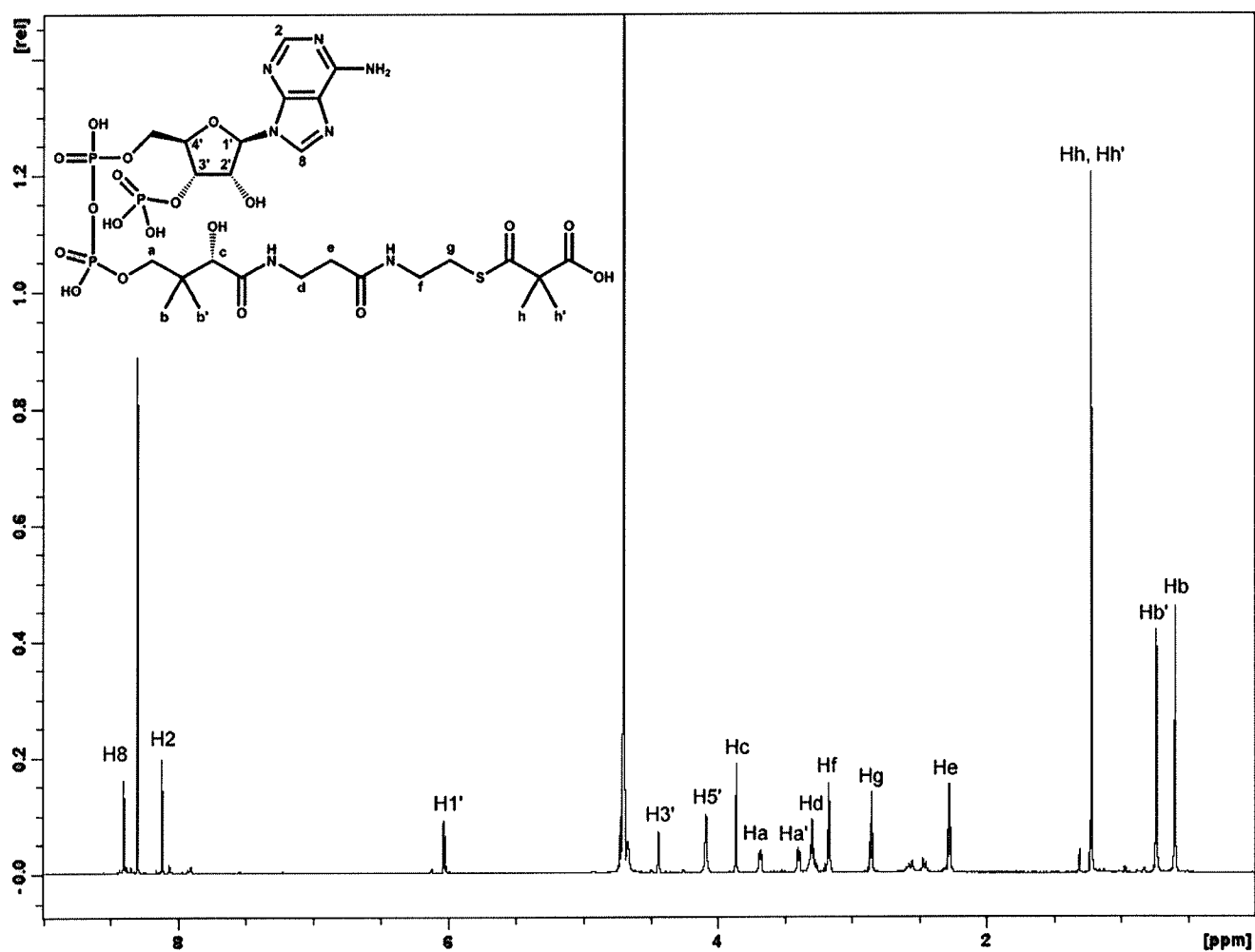
Figure 1: ^1\text{H} -NMR spectrum of purified dimethylmalonyl-CoA.
