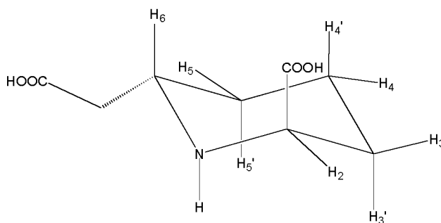
(2 S ,6 S )-6-(carboxymethyl)piperidine-2-carboxylic acid
