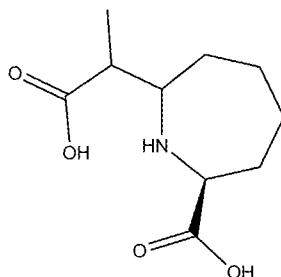
(2 S )-7-(1-carboxyethyl)azepane-2-carboxylic acid
