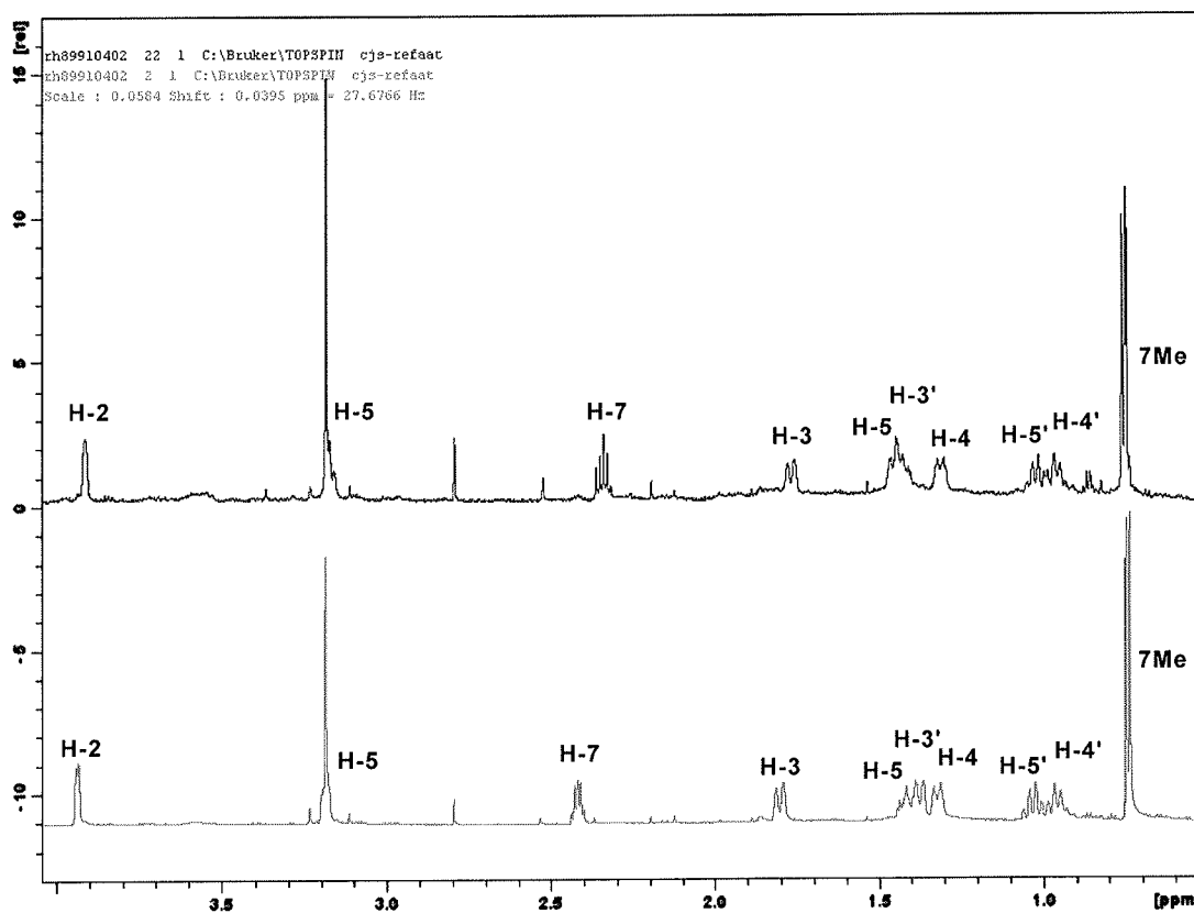
Figure 33: ^1\text{H} -NMR spectra for compound 20 (bottom) and 21 (top).
