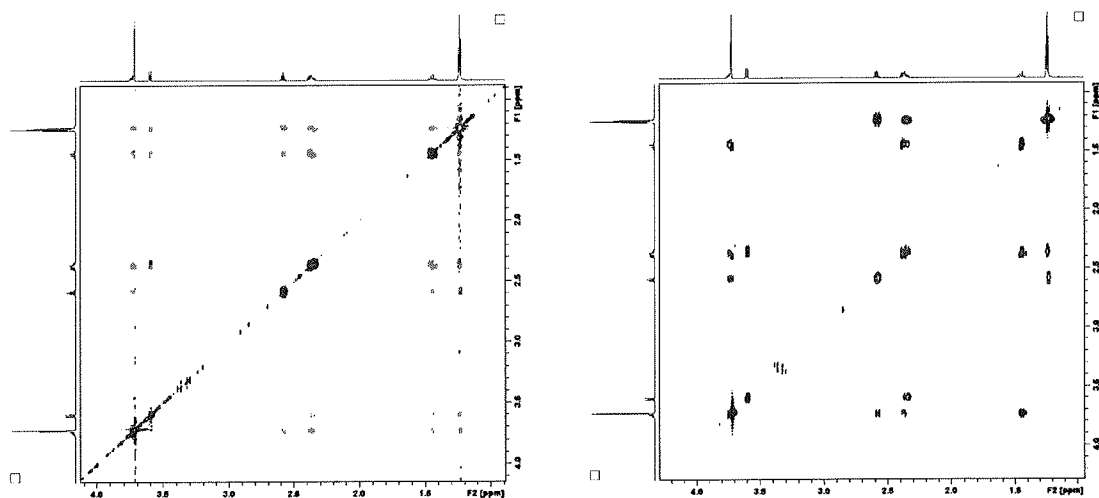
Figure 56: COSY and NOESY spectrum of Compound 30 .
