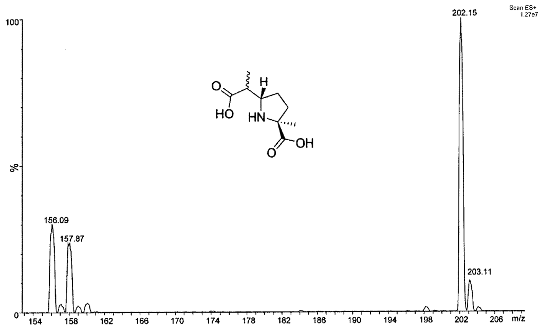
Figure 47: MS spectrum for compound 27
