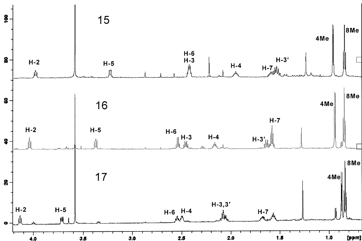
Figure 24: ^1\text{H} -NMR spectra for compounds 15 (top), 16 (middle) and 17 (bottom).
