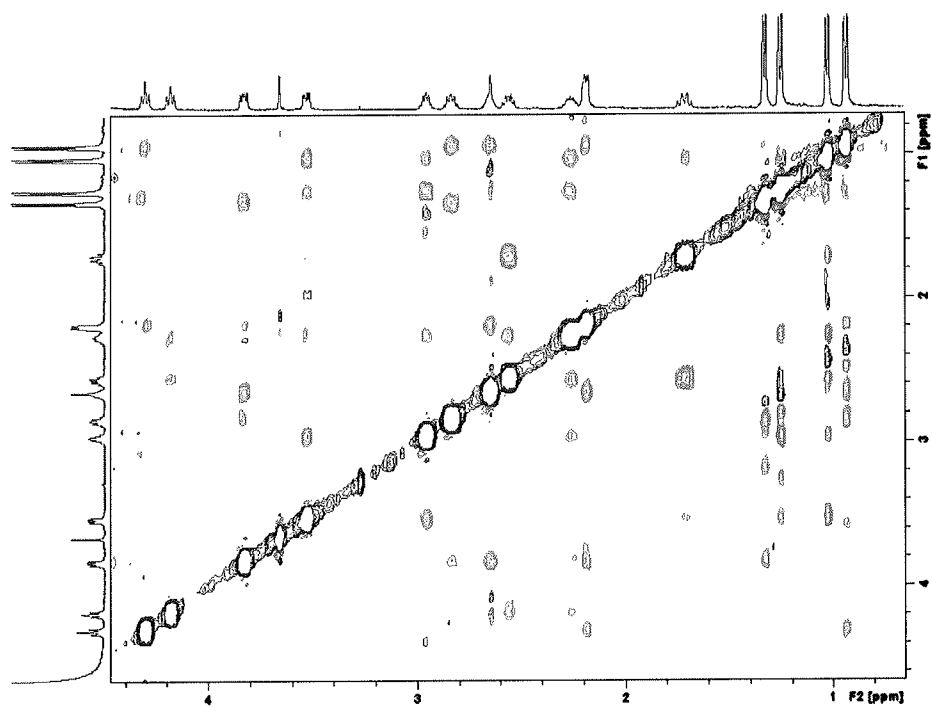
Figure 12: 2D NOESY spectrum for a mixture of compounds 7 and 8 .
