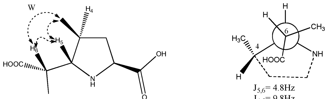
(2 S ,4 S ,5 S )-5-(( S )-1-carboxyethyl)-4-methylpyrrolidine-2-carboxylic acid
