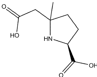
(2 S )-5-(carboxymethyl)-5-methylpyrrolidine-2-carboxylic acid
