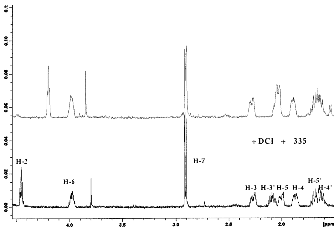
Figure 30: ^1\text{H} -NMR spectra of compound 19 (top) and after addition of deuterium chloride and increasing the temperature to 335 K (bottom).
