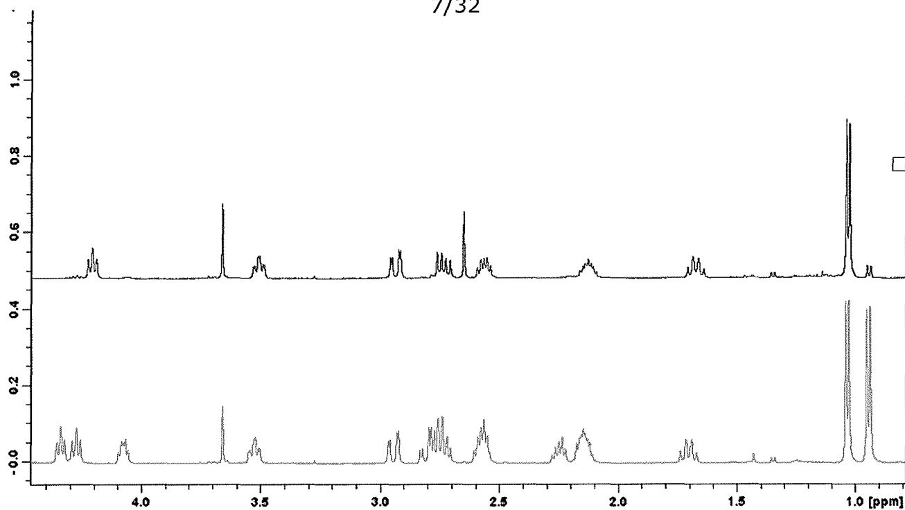
Figure 8: ^1\text{H} -NMR spectra for compounds 4 (top) and 5 (bottom, as a mixture with 4 ), (500MHz, \text{D}_2\text{O} )
