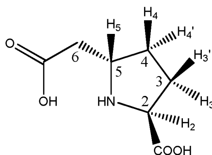
(2 S ,5 S )-5-(carboxymethyl)pyrrolidine-2-carboxylic acid
