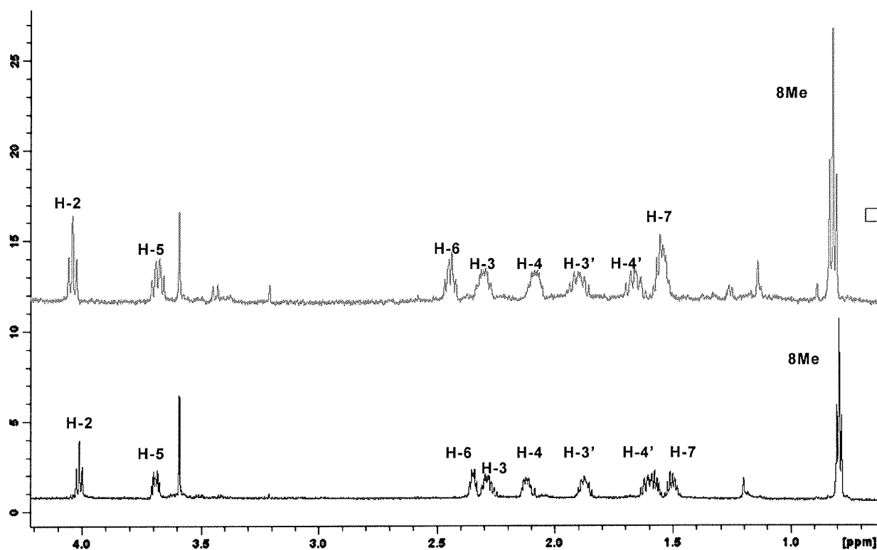
Figure 22: ^1\text{H} -NMR spectra for compounds 13 ( top) and 14 (bottom).
