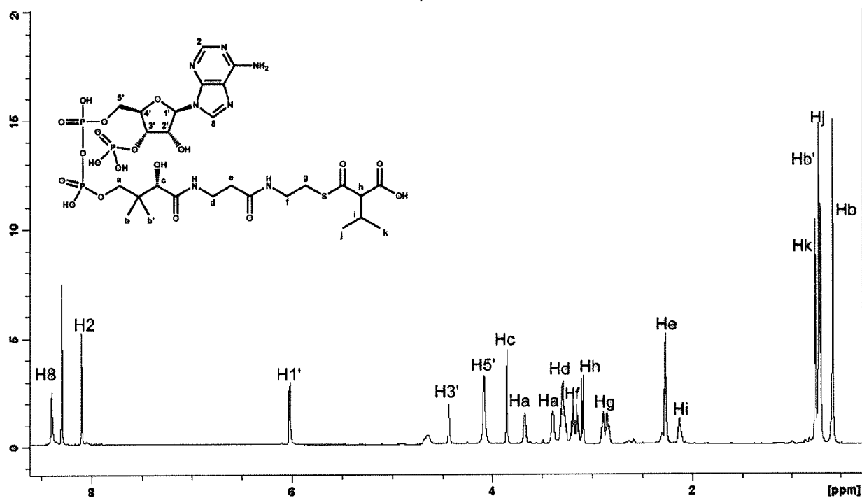
Figure 2: ^1\text{H} -NMR spectrum of purified isopropylmalonyl-CoA.
