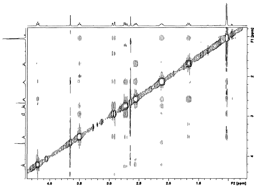
Figure 9: 2D NOESY spectrum for compound 4 , (500MHz, \text{D}_2\text{O} )
