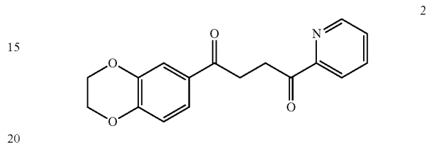
1-(2,3-dihydrobenzo[b][1,4]dioxin-6-yl)-4-(pyridin-2-yl)butane-1,4-dione 2
