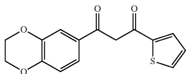
1-(2,3-dihydrobenzo[b][1,4]dioxin-6-yl)-3-(thiophen-2-yl)propane-1,3-dione 16
