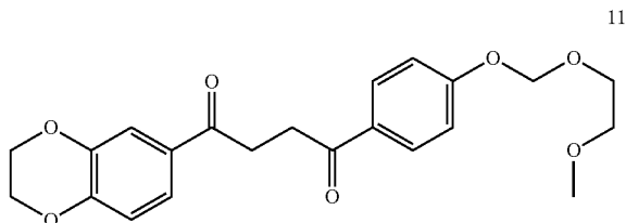
1-(2,3-dihydrobenzo[b][1,4]dioxin-6-yl)-4-(4-((2-methoxyethoxy)methoxy)phenyl)butane-1,4-dione 11
