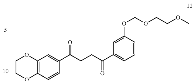
1-(2,3-dihydrobenzo[b][1,4]dioxin-6-yl)-4-(3-((2-methoxyethoxy)methoxy)phenyl)butane-1,4-dione 12
