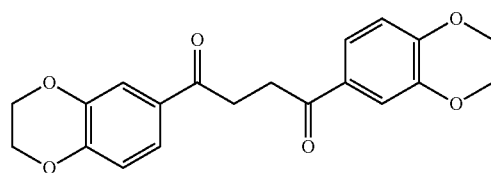
1,4-bis(2,3-dihydrobenzo[b][1,4]dioxin-6-yl)butane-1,4-dione 14
