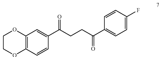
1-(2,3-dihydrobenzo[b][1,4]dioxin-6-yl)-4-(4-fluorophenyl)butane-1,4-dione 7
