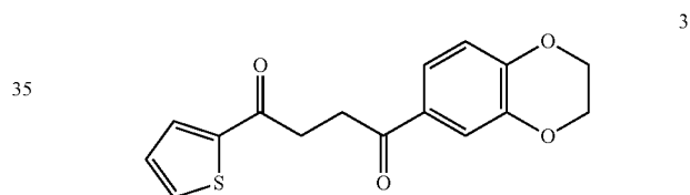
1-(2,3-dihydrobenzo[b][1,4]dioxin-6-yl)-4-(thiophen-2-yl)butane-1,4-dione 3
