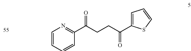
1-(pyridin-2-yl)-4-(thiophen-2-yl)butane-1,4-dione 5
