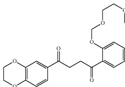
1-(2,3-dihydrobenzo[b][1,4]dioxin-6-yl)-4-(2-((2-methoxyethoxy)methoxy)phenyl)butane-1,4-dione 13
