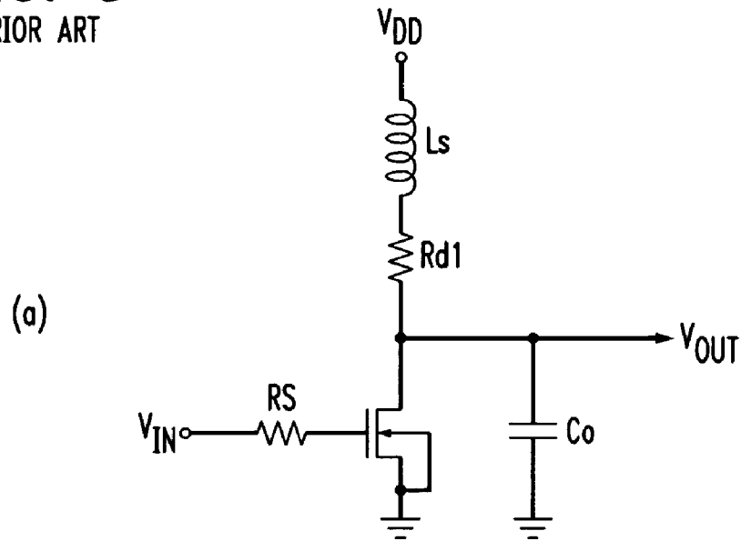
TYPICAL SHUNT PEAKED AMPLIFIER
