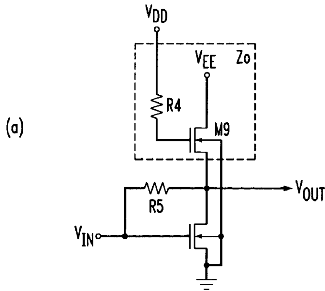
COMMON SOURCE STAGE WITH FEEDBACK RESISTOR
