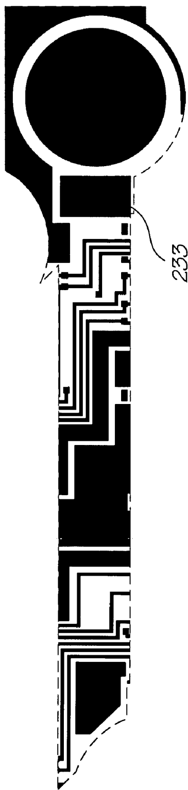
Metal 2 mask
