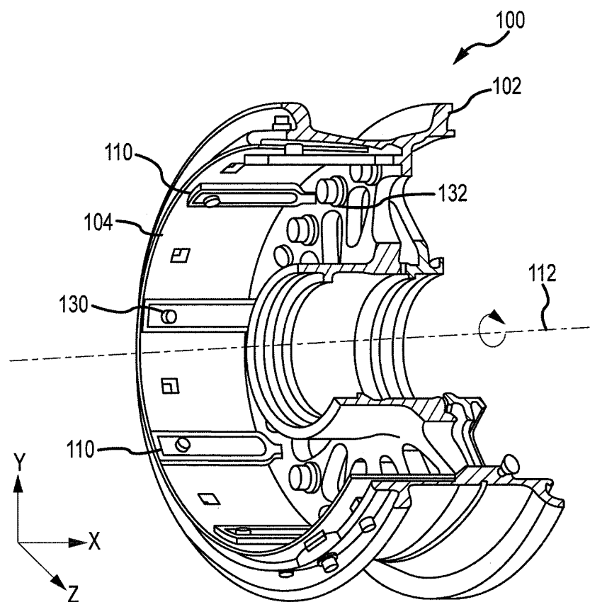
FIG. 1 (PRIOR ART)
