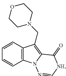
5-(morpholinomethyl)-[1,2,4]triazino[1,6-a]indol-4(3H)-one
