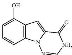
6-hydroxy-[1,2,4]triazino[1,6-a]indol-4(3H)-one
