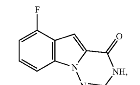
6-fluoro-[1,2,4]triazino[1,6-a]indol-4(3H)-one
