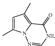
5,7-dimethylpyrrolo[2,1-f][1,2,4]triazin-4(3H)-one
