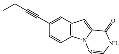
7-(but-1-yn-1-yl)-[1,2,4]triazino[1,6-a]indol-4(3H)-one
