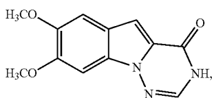
7,8-dimethoxy-[1,2,4]triazino[1,6-a]indol-4(3H)-one
