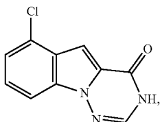
6-chloro-[1,2,4]triazino[1,6-a]indol-4(3H)-one
