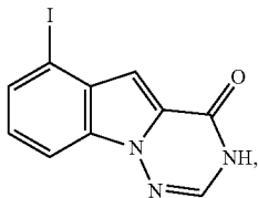
6-iodo-[1,2,4]triazino[1,6-a]indol-4(3H)-one
