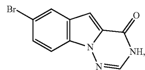
7-bromo-[1,2,4]triazino[1,6-a]indol-4(3H)-one
