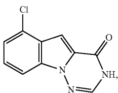
6-chloro-[1,2,4]triazino[1,6-a]indol-4(3H)-one
