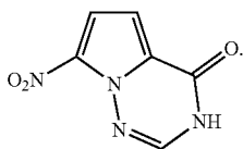
7-nitropyrrrolo-[2,1-f][1,2,4]triazino-4(3H)-one
