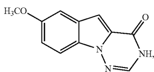
7-methoxy-[1,2,4]triazino[1,6-a]indol-4(3H)-one
