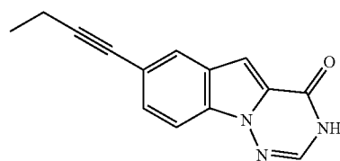
7-(but-1-yn-1-yl)-[1,2,4]triazino[1,6-a]indol-4(3H)-one
