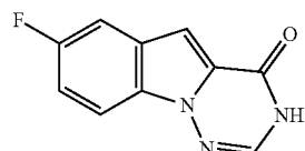
7-fluoro-[1,2,4]triazino[1,6-a]indol-4(3H)-one
