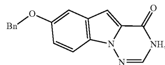
7-(benzyloxy)-[1,2,4]triazino[1,6-a]indol-4(3H)-one
