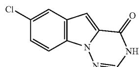
7-chloro-[1,2,4]triazino[1,6-a]indol-4(3H)-one
