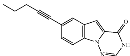
7-(pent-1-yn-1-yl)-[1,2,4]triazino[1,6-a]indol-4(3H)-one
