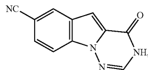
4-oxo-3,4-dihydro-[1,2,4]triazino[1,6-a]indole-7-carbonitrile
