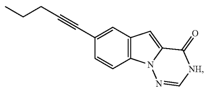
7-(pent-1-yn-1-yl)-[1,2,4]triazino[1,6-a]indol-4(3H)-one
