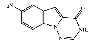
7-amino-[1,2,4]triazino[1,6-a]indol-4(3H)-one
