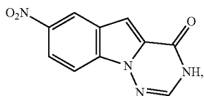
7-nitro-[1,2,4]triazino[1,6-a]indol-4(3H)-one
