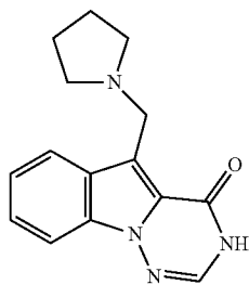
5-(pyrrolidin-1-ylmethyl)-[1,2,4]triazino[1,6-a]indol-4(3H)-one
