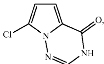
7-chloropyrrolo-[2,1-f][1,2,4]triazino-4(3H)-one
