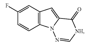
7-fluoro-[1,2,4]triazino[1,6-a]indol-4(3H)-one
