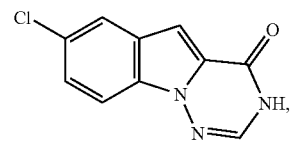
7-chloro-[1,2,4]triazino[1,6-a]indol-4(3H)-one
