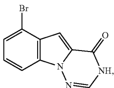
6-bromo-[1,2,4]triazino[1,6-a]indol-4(3H)-one
