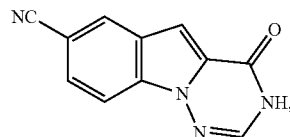
4-oxo-3,4-dihydro-[1,2,4]triazino[1,6-a]indole-7-carbonitrile
