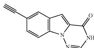
7-ethynyl-[1,2,4]triazino[1,6-a]indol-4(3H)-one
