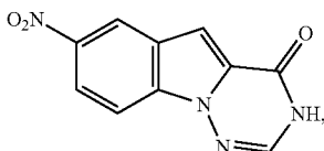
7-nitro-[1,2,4]triazino[1,6-a]indol-4(3H)-one
