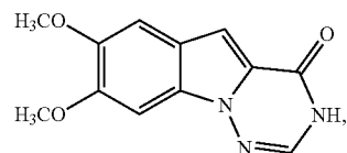
7-8-dimethoxy-[1,2,4]triazino[1,6-a]indol-4(3H)-one
