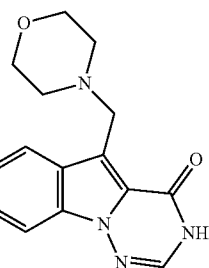
5-(morpholinomethyl)-[1,2,4]triazino[1,6-a]indol-4(3H)-one
