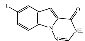
7-iodo-[1,2,4]triazino[1,6-a]indol-4(3H)-one
