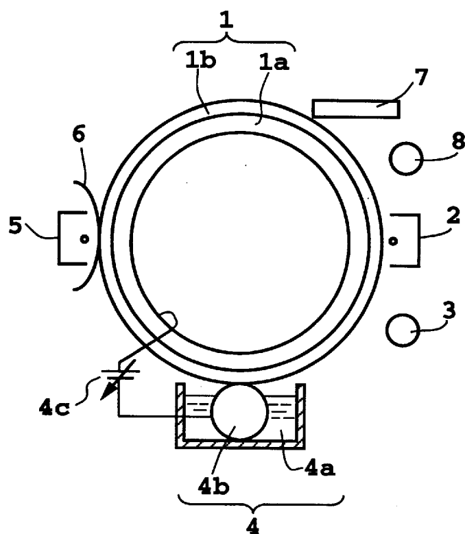
FIG. 1 (PRIOR ART)
