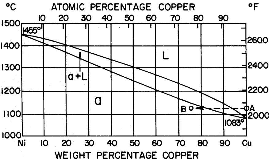
COPPER-NICKEL PHASE DIAGRAM
