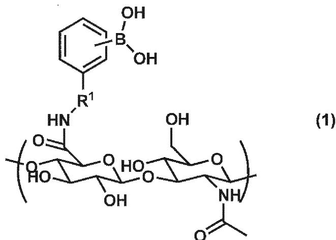
[Chemical Formula 4]
