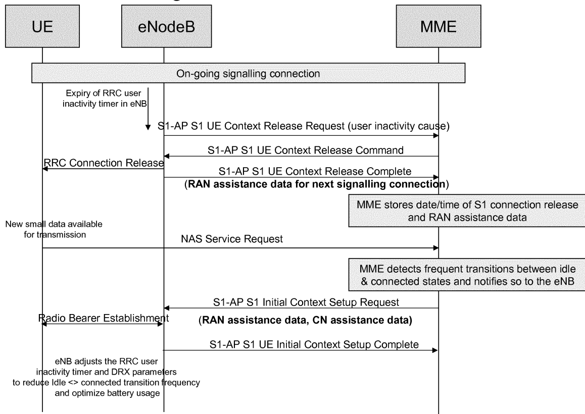
Fig 3- MME assistance info for eNB
