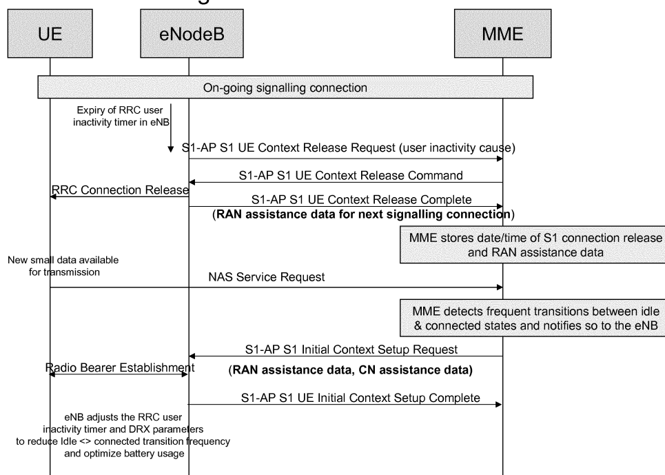
Fig 3- MME assistance info for eNB
