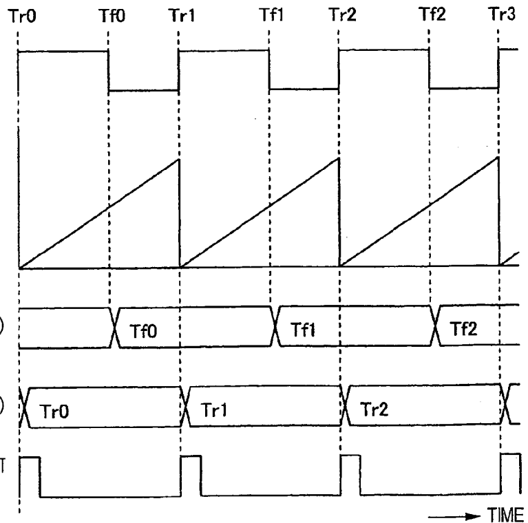
FIG.7A PULSE SIGNAL 6
