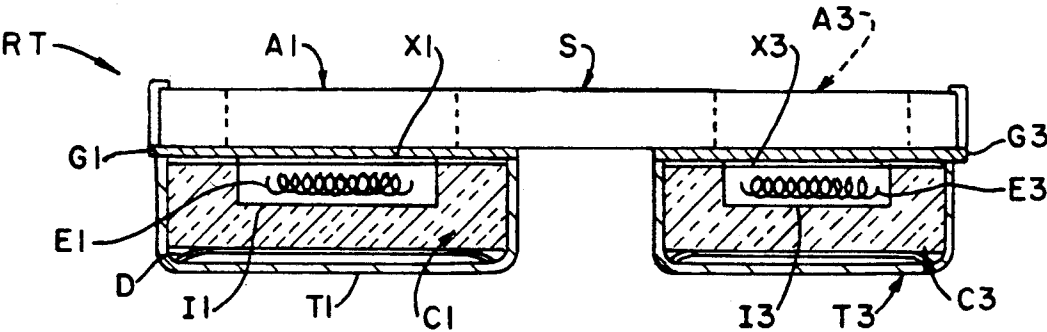
FIG. 2. PRIOR ART.
