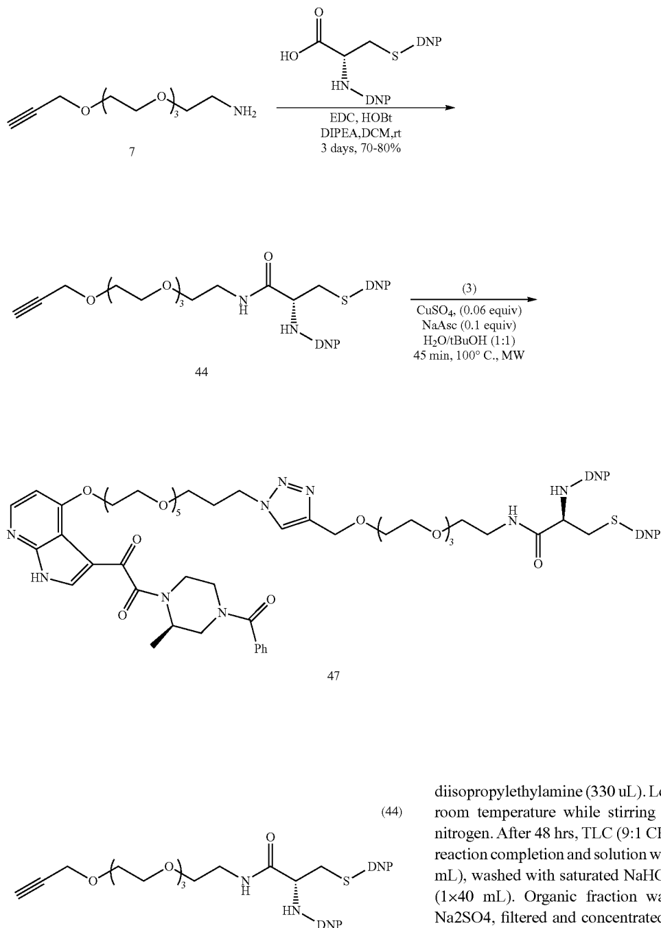
Supplementary Scheme 2. Representative Synthesis of ARM—H type (47) molecules with DNP containing Amino Acids
