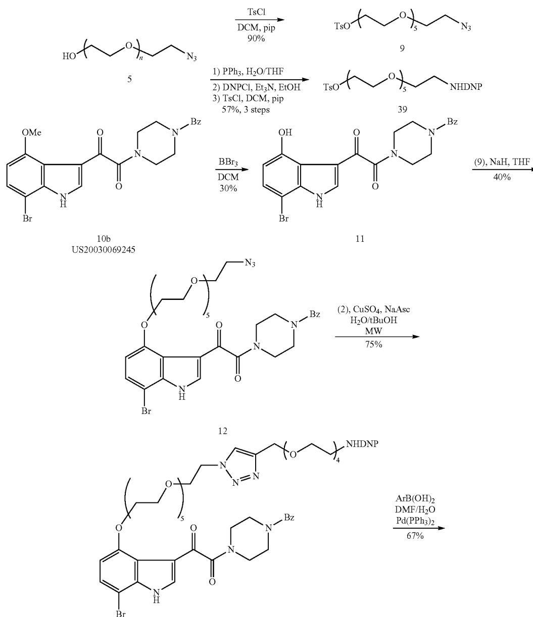
Supplementary Scheme 4. Representative Synthesis of ARM—H type (14) and type (28) molecules
