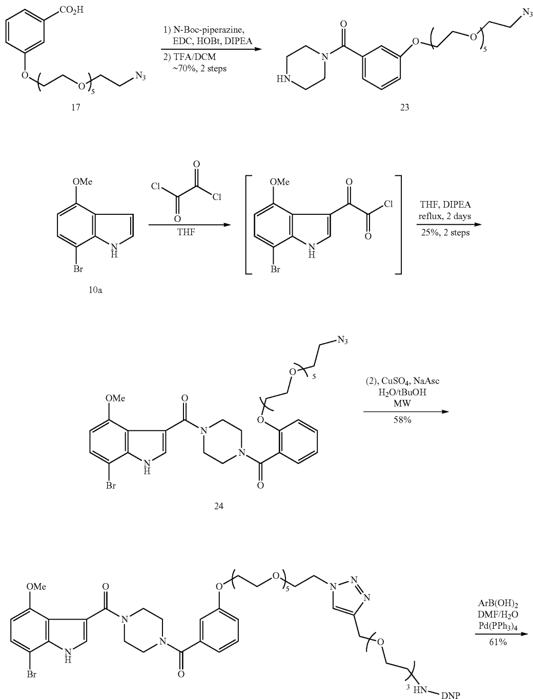
Supplementary Scheme 6. Representative Synthesis of ARM—H type (26) molecules
