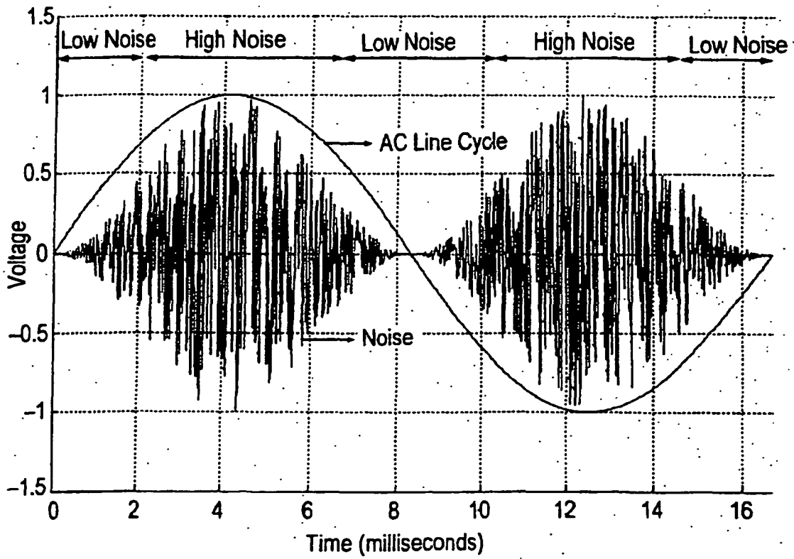
Example of Noise Variation with AC Line Cycle Phase
