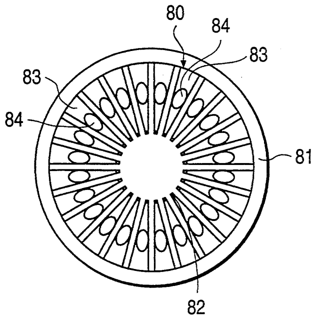
FIG. 13 PRIOR ART
