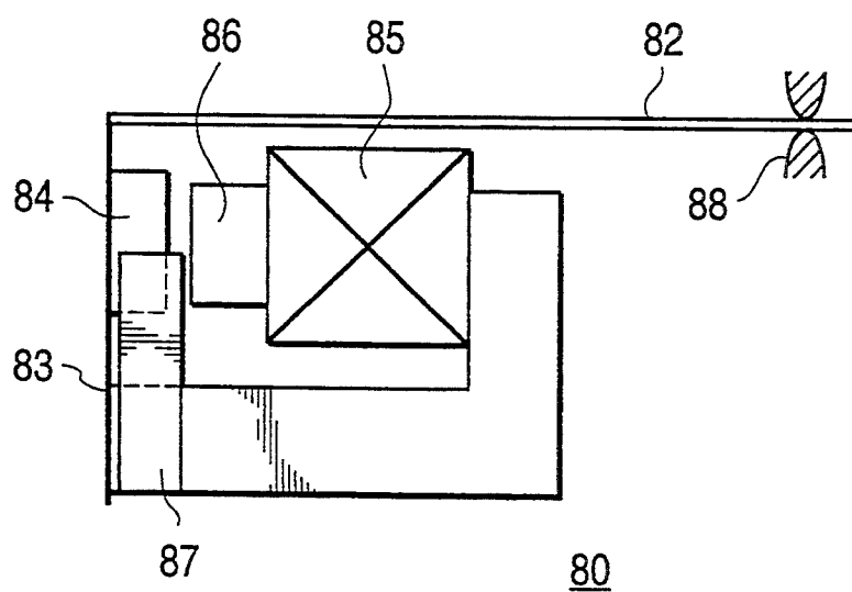
FIG. 14 PRIOR ART
