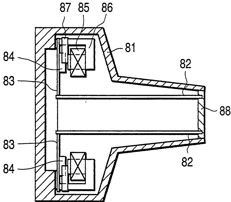
FIG. 12 PRIOR ART
