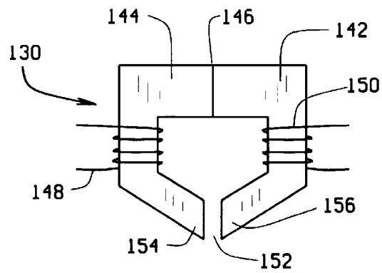
FIG. 4 PRIOR ART
