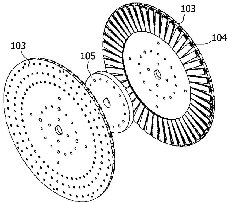
FIG.11 (PRIOR ART)
