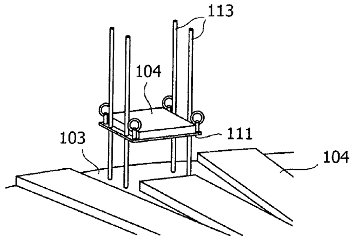
FIG.10 (PRIOR ART)
