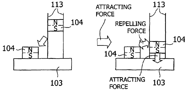
FIG.13 (PRIOR ART)
