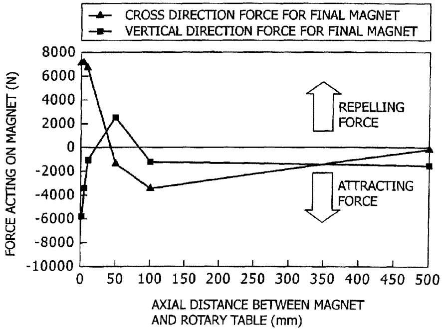
FIG.13 (PRIOR ART)
