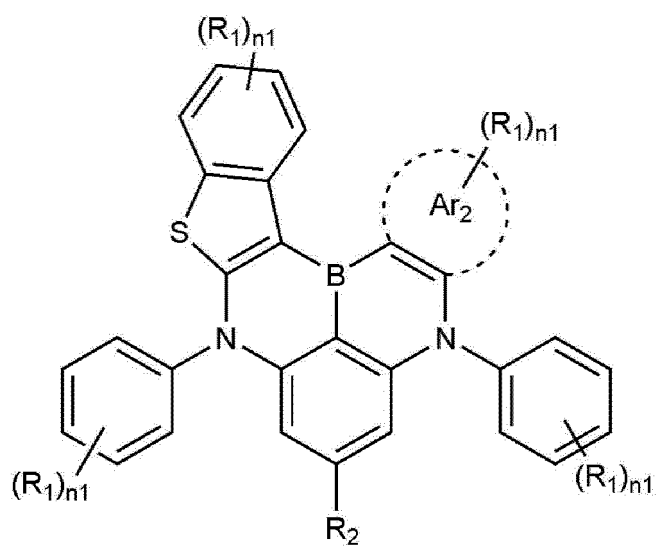
[Chemical Formula 1-2]
