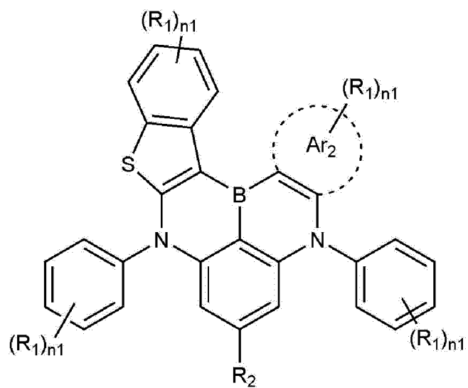
[Chemical Formula 1-3]
