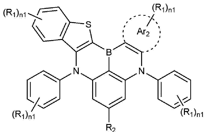
[Chemical Formula 1-1]
