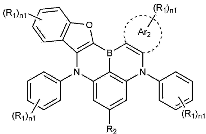
[Chemical Formula 1-4]
