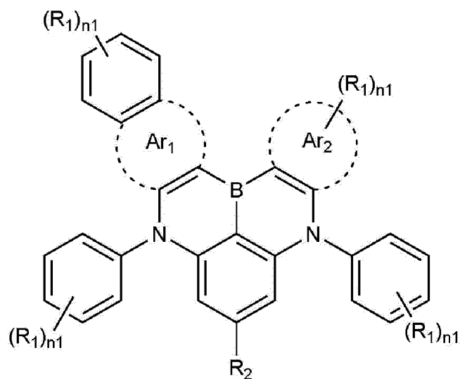
[Chemical Formula 1]
