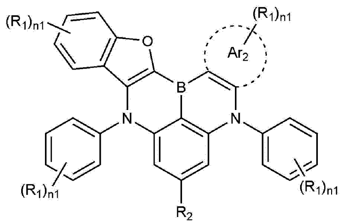
[Chemical Formula 1-3]
