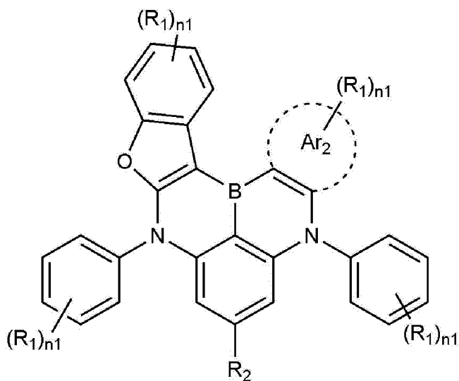
[Chemical Formula 1-4]
