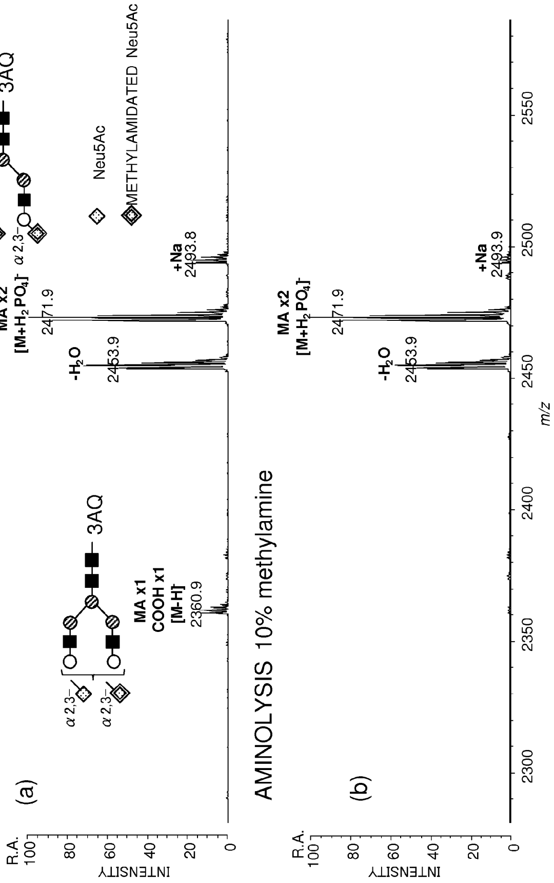
FIG. 10 AMINOLYSIS 1% methyllamine
