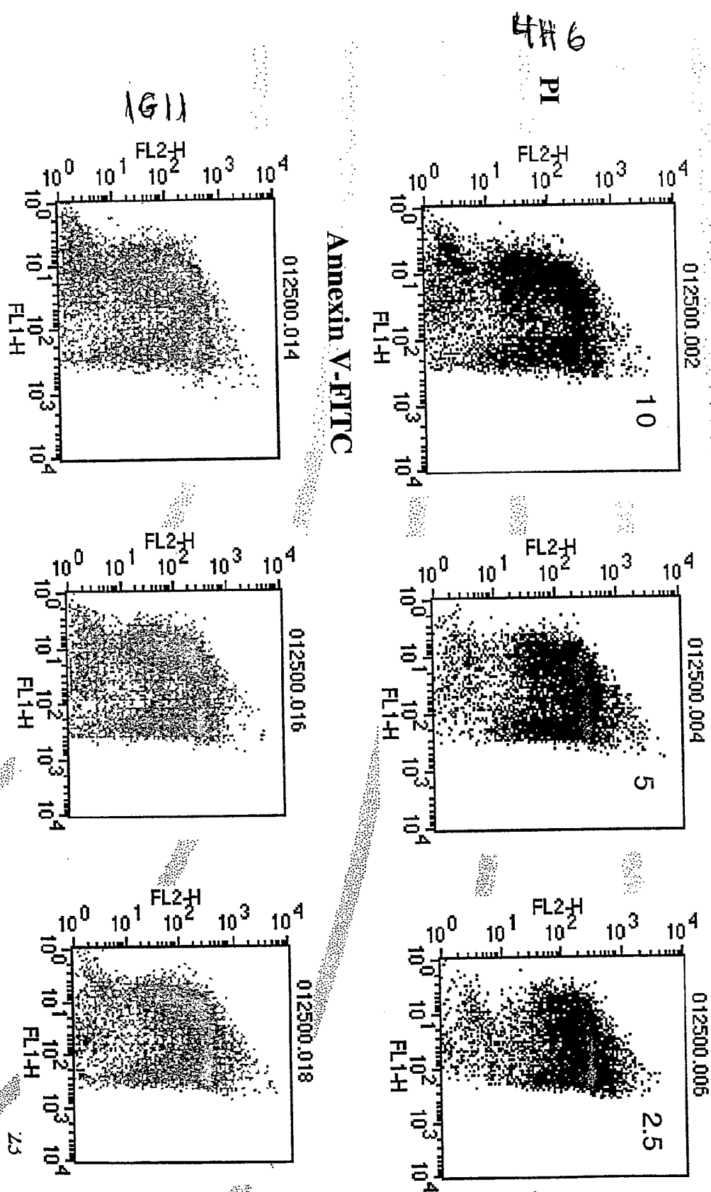
Apoptosis assay by Annexin V staining FIG. 5
