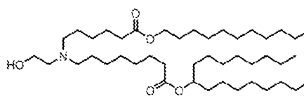
Moderna Lipid H
