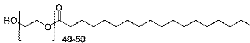
PEG Stearate (Compound I)
