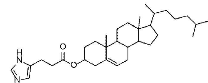
Moderna Lipid H
