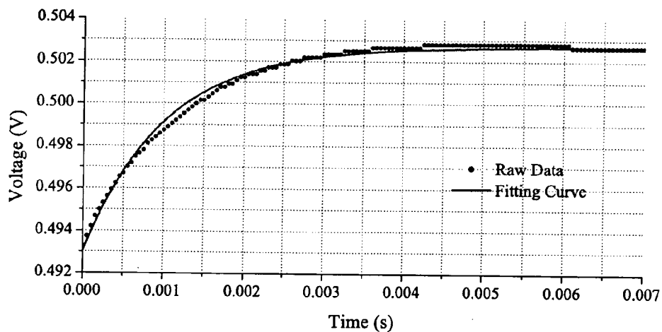
Figure 7. Flow sensor thermal time constant measurement
