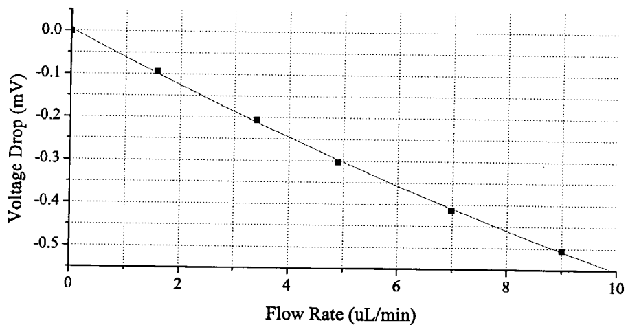
Figure 5. Flow sensor characteristic for air flow.
