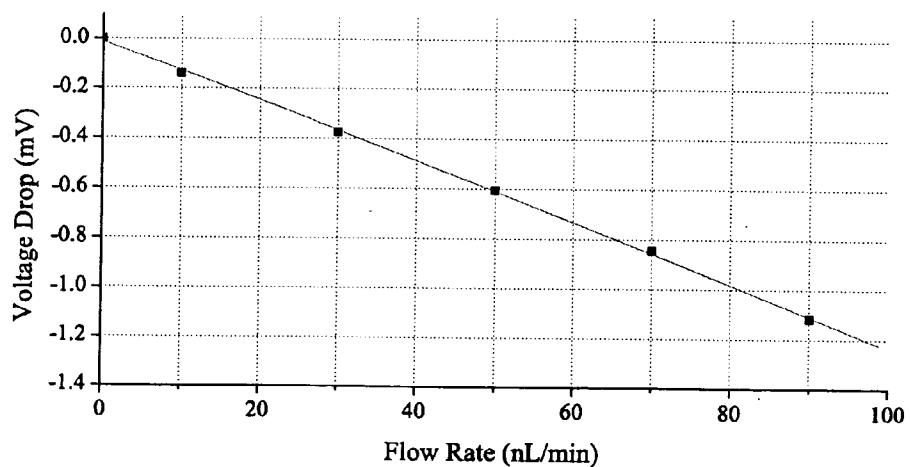
Figure 6. Flow sensor characteristic for water.
