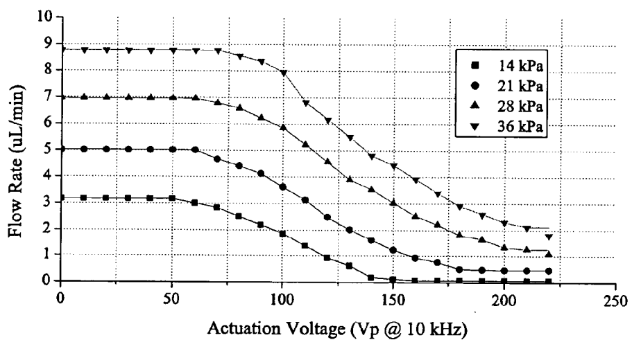
Figure 8. Flow rate vs. actuation voltage.
