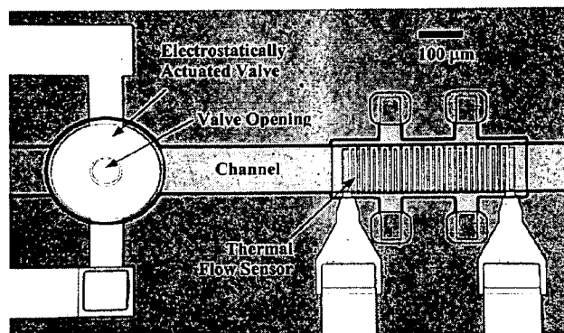
Figure 4. Fabricated Devices
