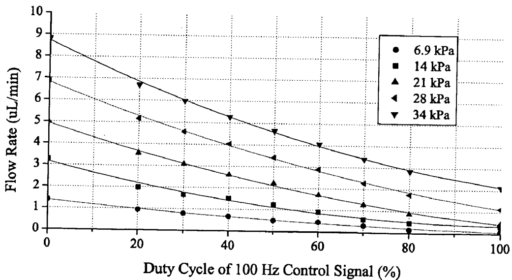
Figure 11. Flow control in PWM mode.
