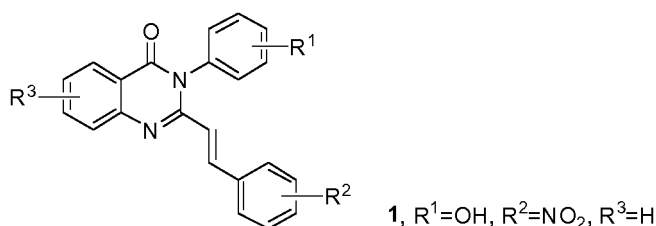
Scheme 1. One representative quinazolinone compound.
