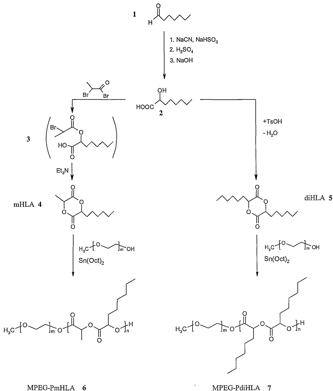
Scheme 5
