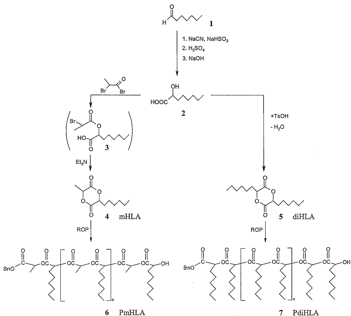
Scheme 4
