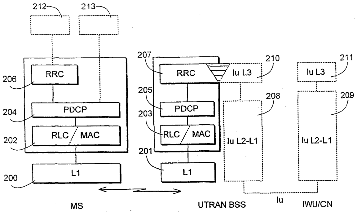
Fig. 2 PRIOR ART
