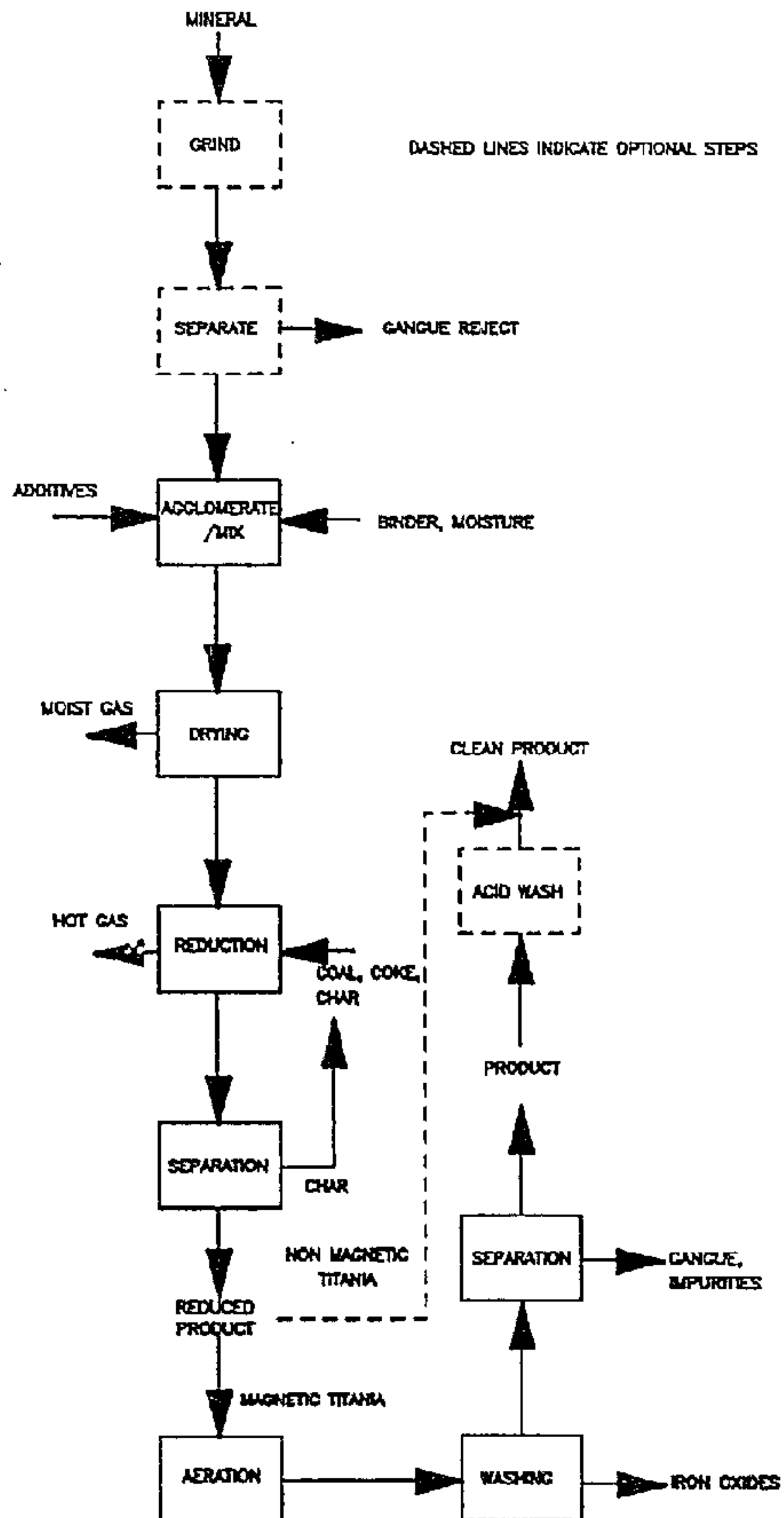
FLWSHEET OF PROCESS FOR PRODUCING ACID SOLUBLE TITANIA
