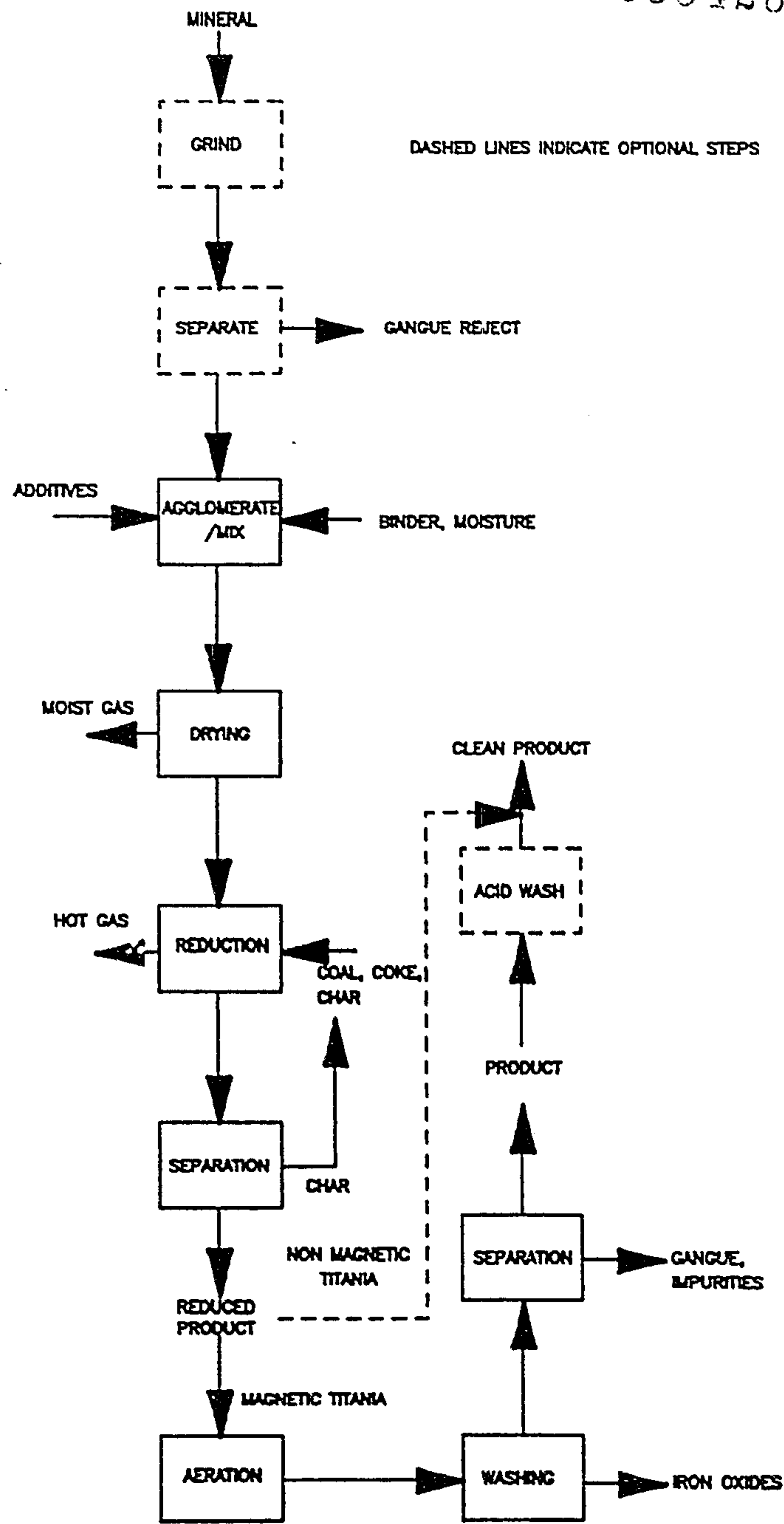
FIGURE 1: FLOWSHEET OF PROCESS FOR PRODUCING ACID SOLUBLE TITANIA
