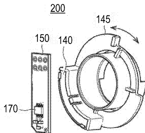
First position (throttle is fully closed)
