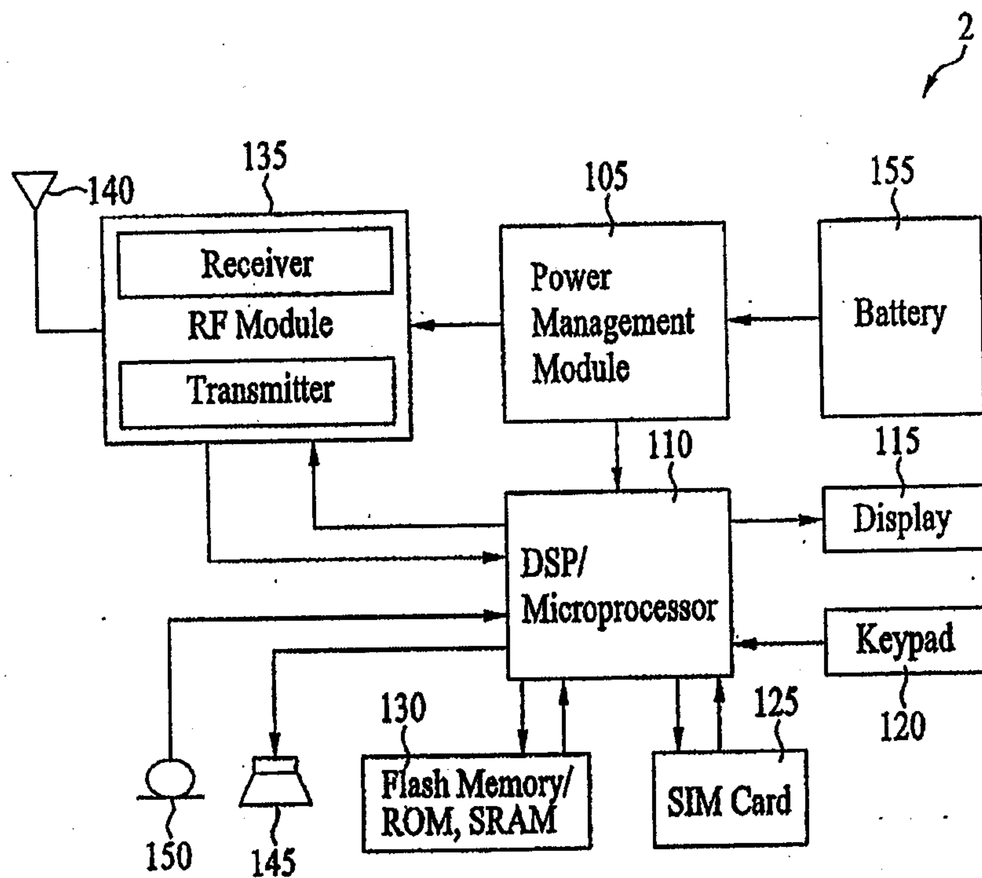
FIG. 17 MOBILE STATION/ACCESS TERMINAL
