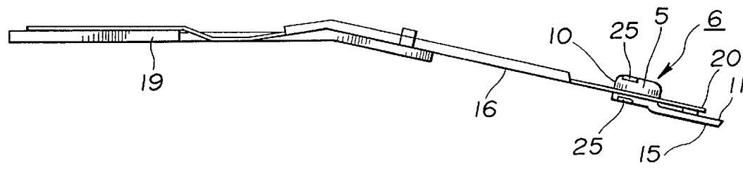
FIG.2 (PRIOR ART)
