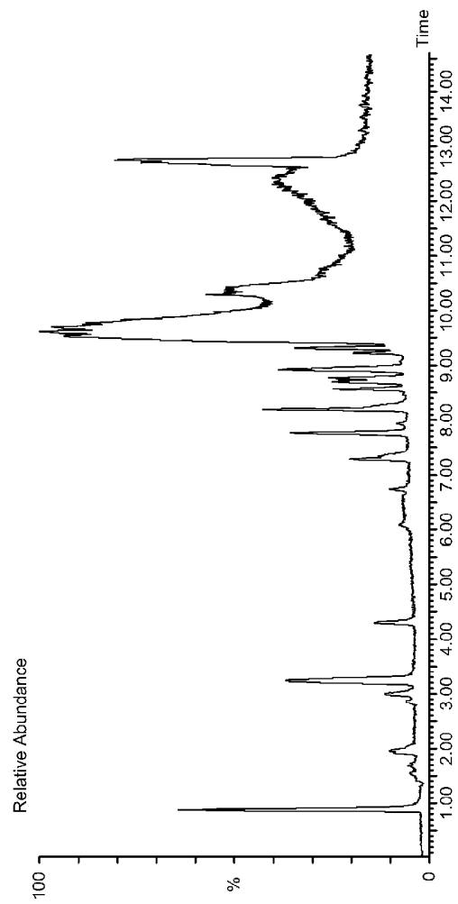
Total Ion Chromatogram of Feed Sample
