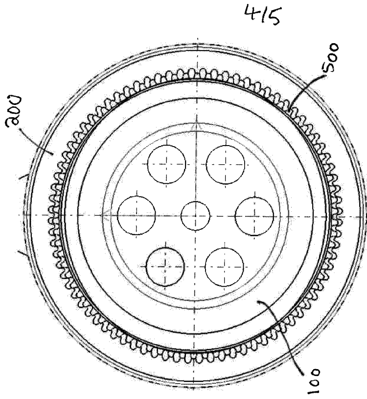
Output Gear
