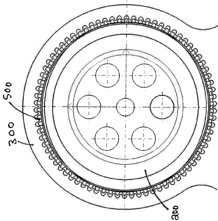
Earth Gear
