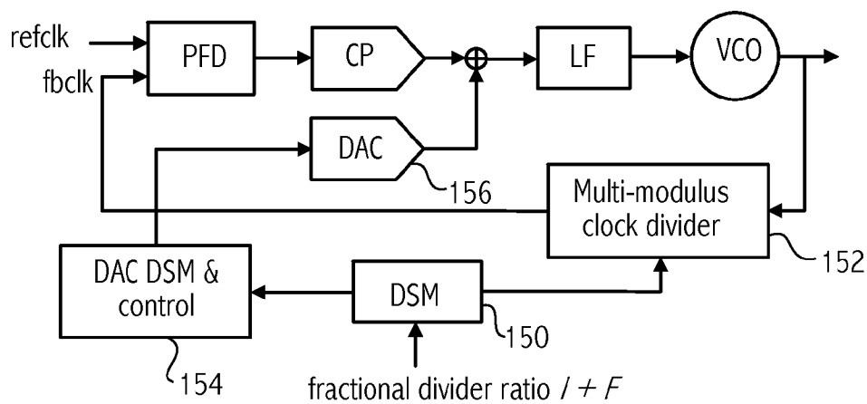
FIG. 1C (Prior Art)
