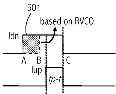
fbclk leads refclk FIG. 5A
