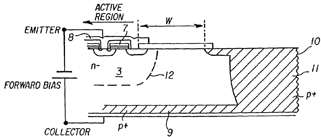
FIG. 24b (Prior Art)
