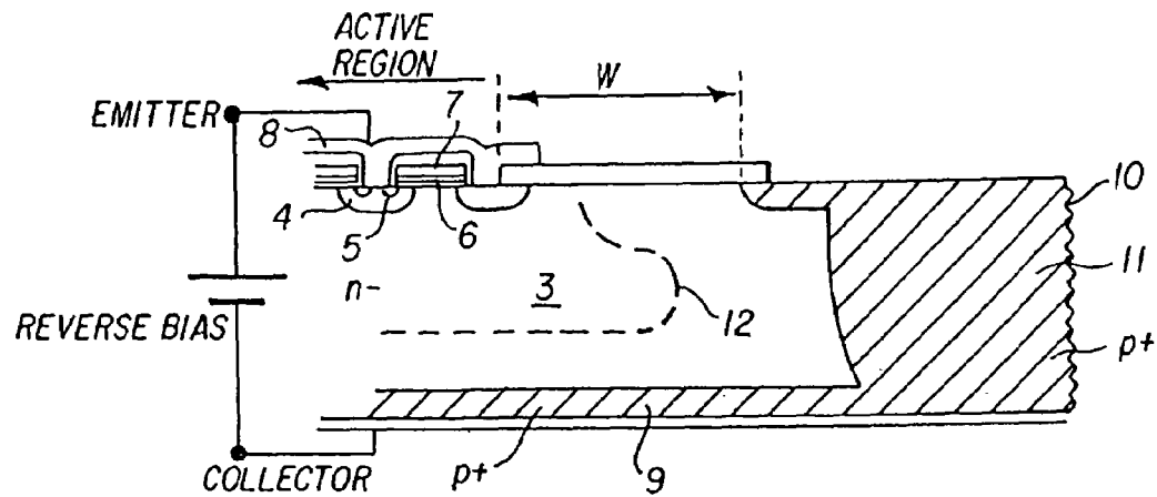
FIG. 24a (Prior Art)
