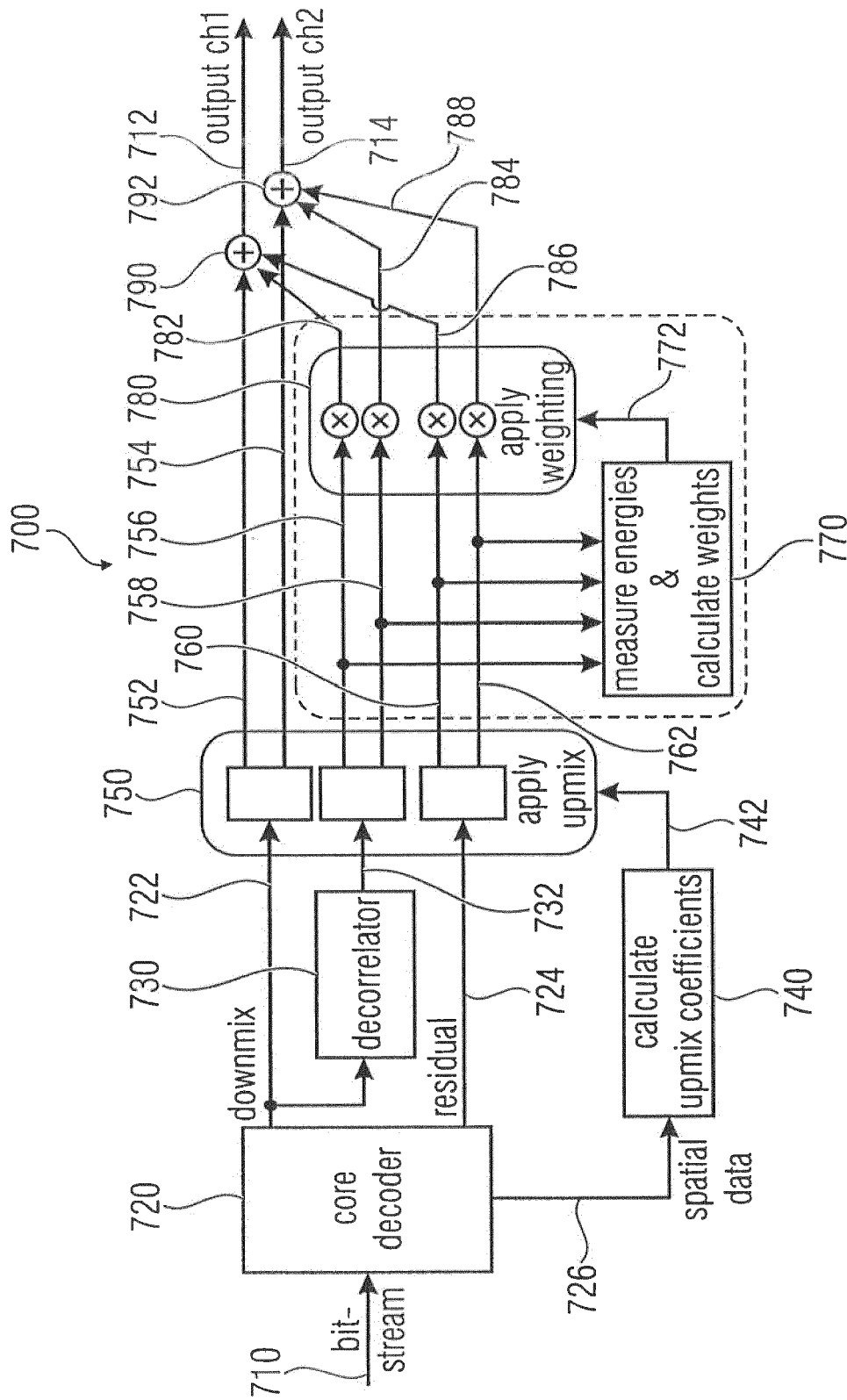
FLOW DIAGRAM OF DECODER FIG 7
