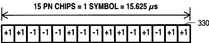
Fig. 3c: PN sequence
