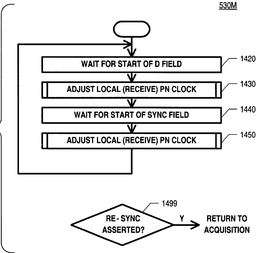
Fig. 14: Flowchart of slow tracking in master.
