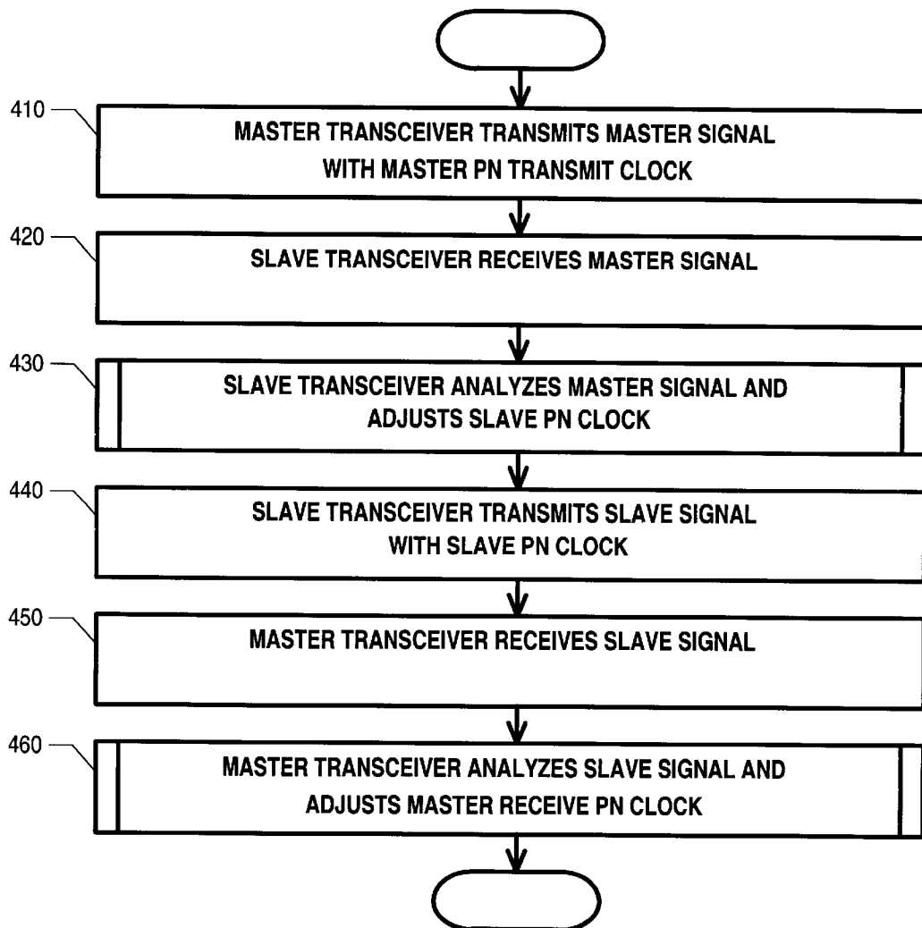
Fig. 4: Flowchart of PN synchronization.
