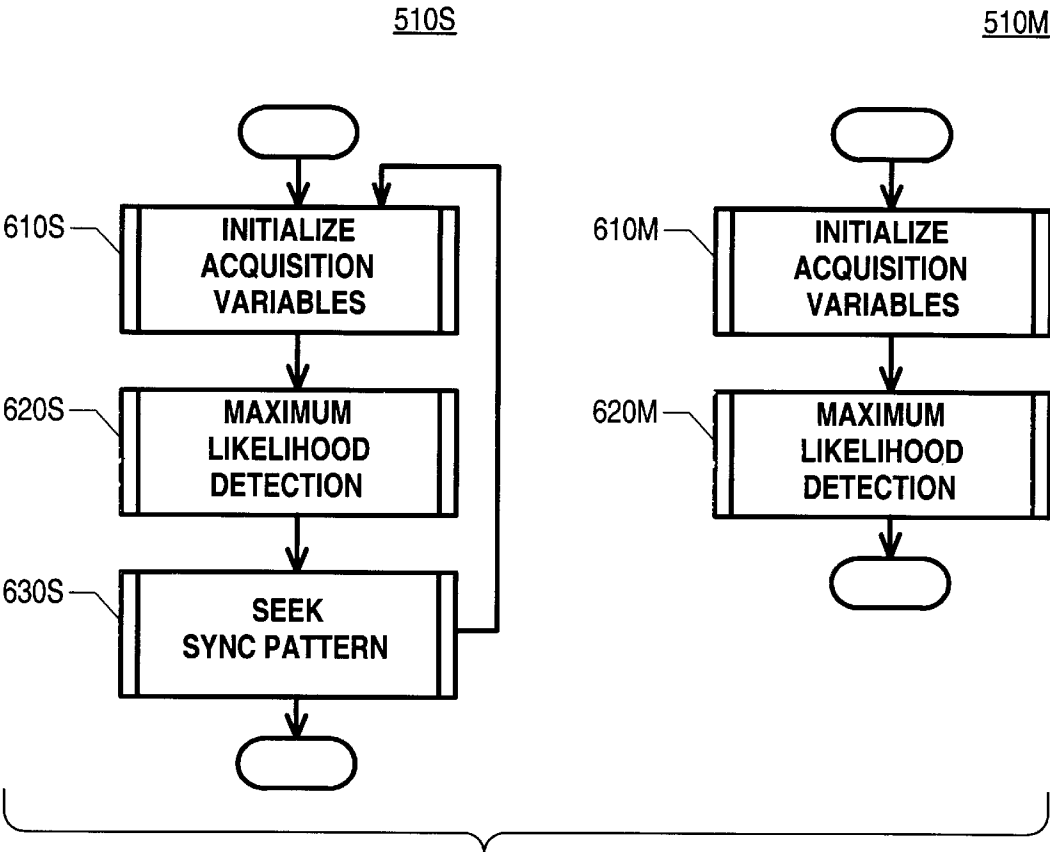
Fig. 6: Acquisition flowchart.
