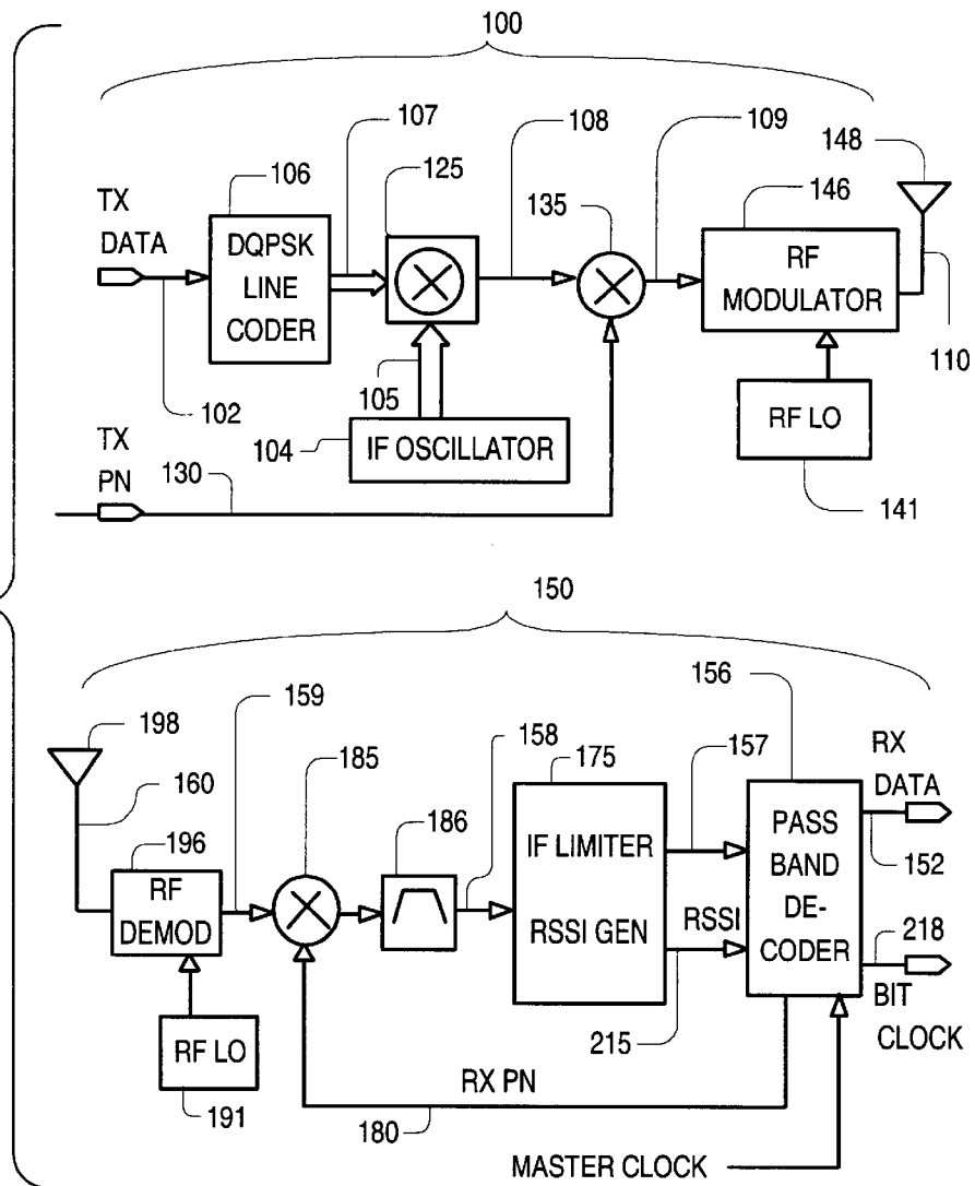
Fig. 1c: DQPSK Spread- spectrum transceiver.
