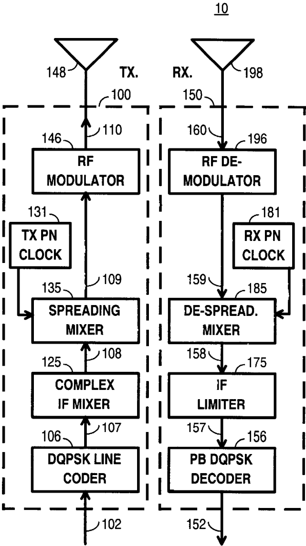
Fig. 1b: DQPSK Spread-spectrum transceiver.
