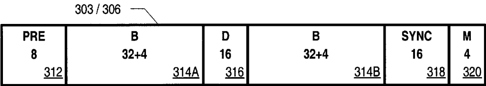
Fig. 3b: Transmit or received frame
