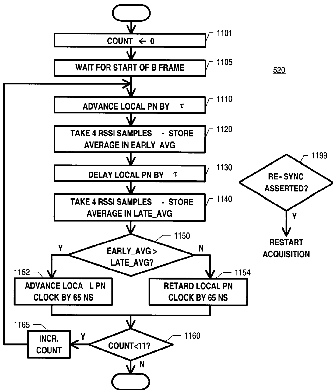
Fig. 11: Fast tracking PN adjustment
