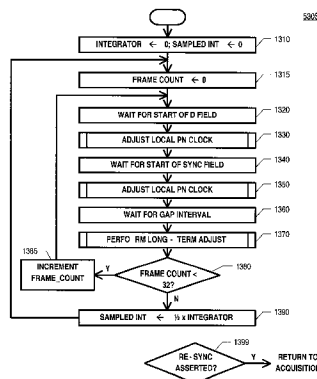
Flowchart of slow tracking in slave.
