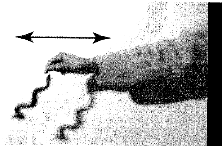
Left : horizontal oscillations of a clump of curly hair. Right : simulation using a simple Super-Helix
