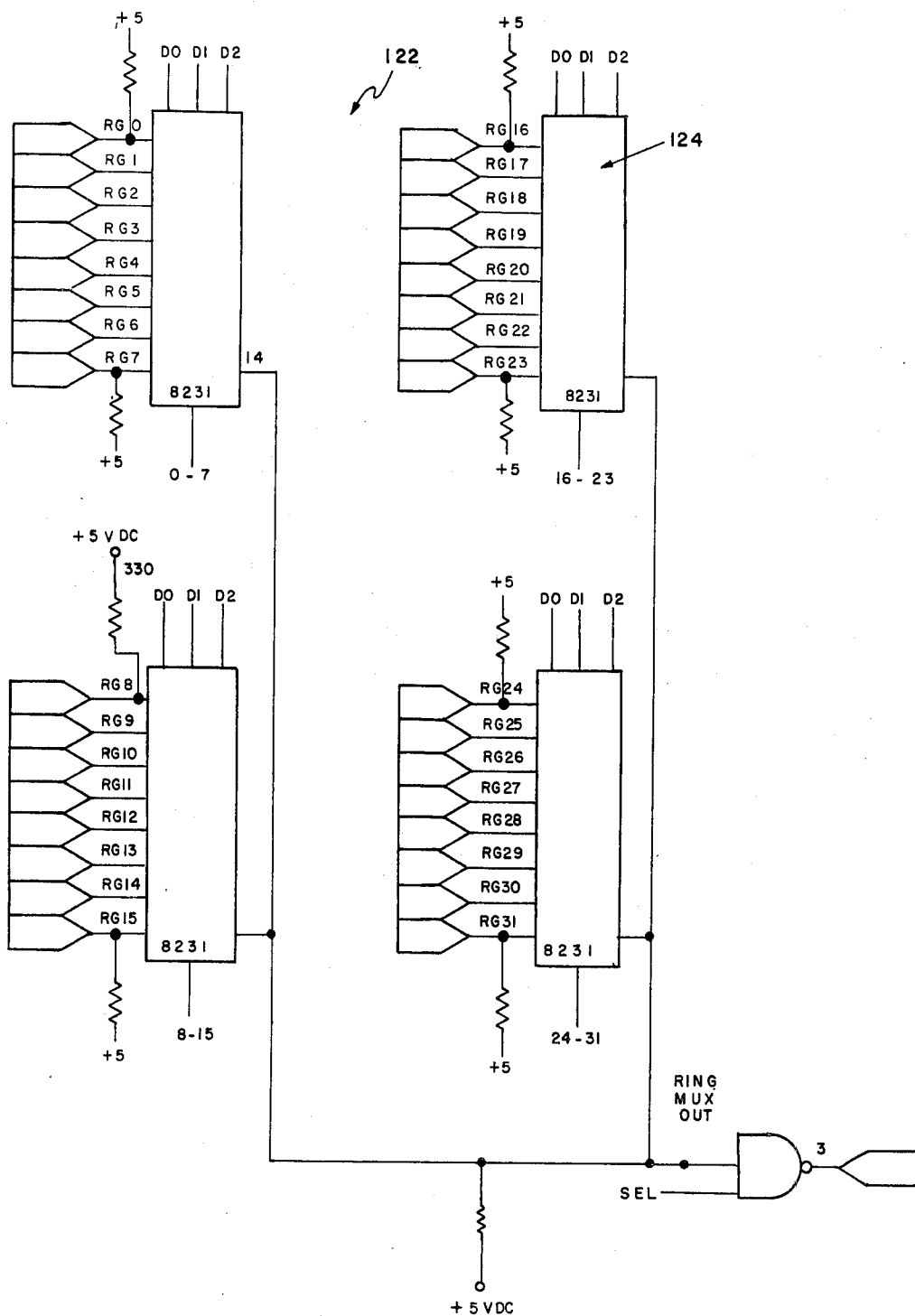
FIG. II RING MUX
