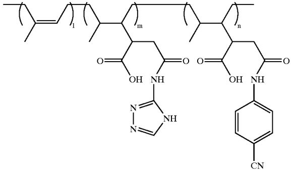
THERMO-REVERSIBLE, CROSSLINKABLE ELASTOMER (8f)
