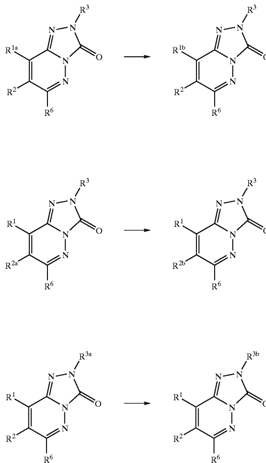
SCHEME 7
