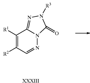
SCHEME 9
