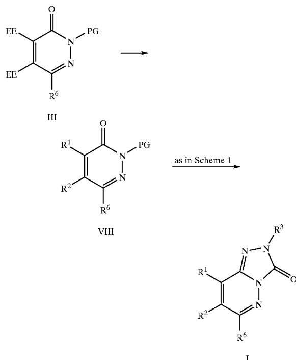
SCHEME 5
