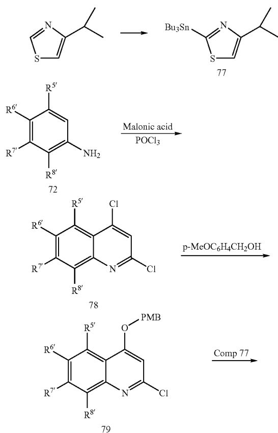
Scheme 17
