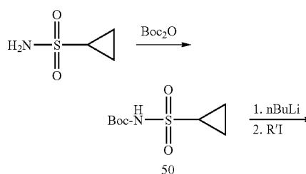
Scheme 9
