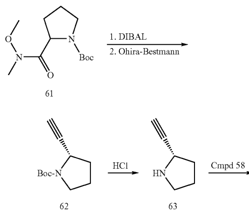
Scheme 13
