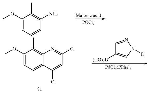
Scheme 18
