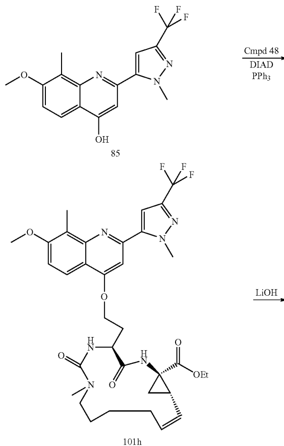
Scheme 28
