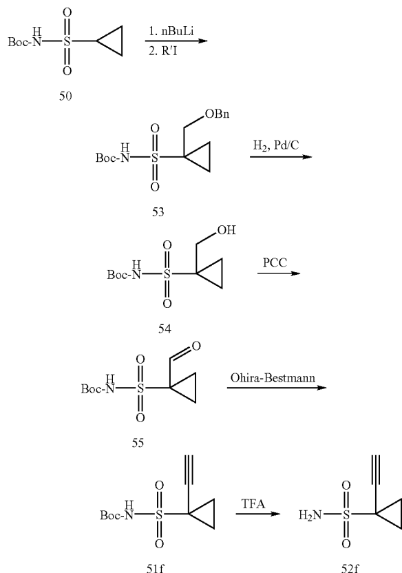
Scheme 10
