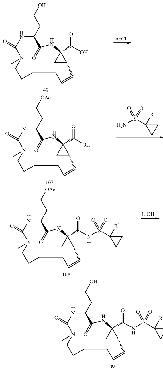
Scheme 26
