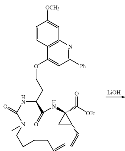
Scheme 5
