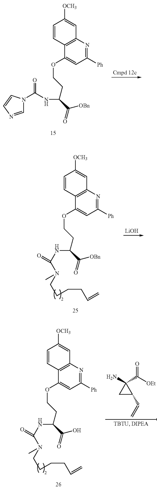
Scheme 6
