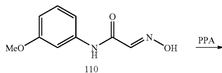
Scheme 27
