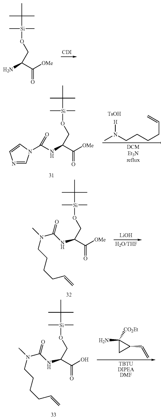
Scheme 7
