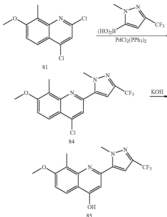
Scheme 19
